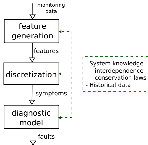
Figure 1: Overview model-based fault diagnosis.
