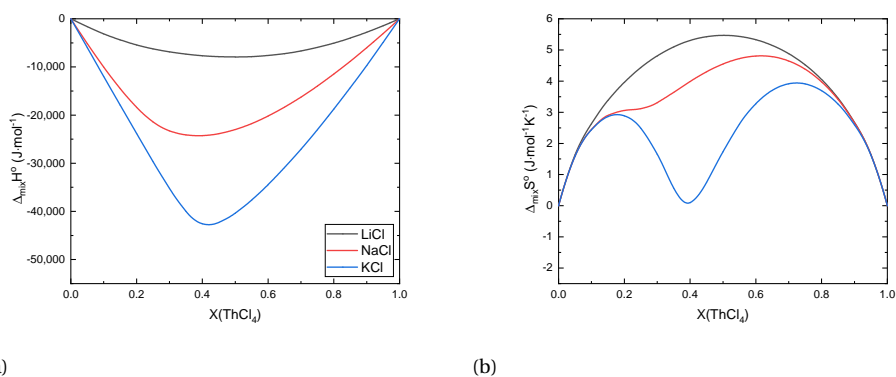
Figure A.4: (a) Enthalpies and (b) entropies of mixing of the (\text{A,Th})\text{Cl}_x liquid solutions calculated at T = 1100\text{ K} .
