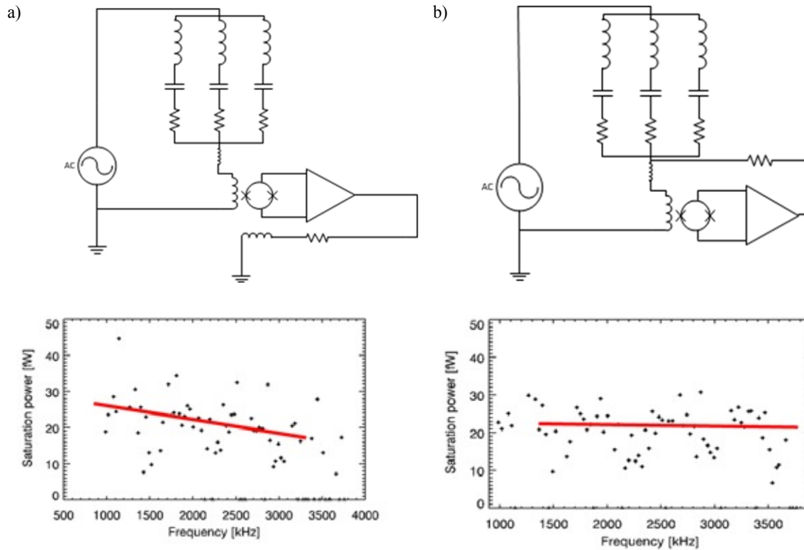
Figure 12. a) schematic of the FDM circuit using the feedback on the feedback coil with the saturation powers as function of resonance frequency; b) Schematic of the FDM circuit using the feedback on the input coil, and therefore screening the common inductance, with the saturation powers as function of resonance frequency
