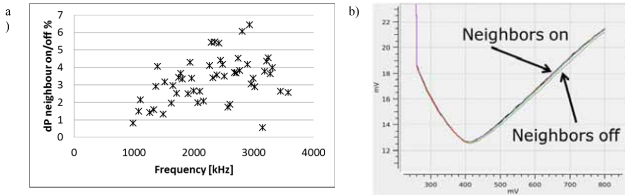
Figure 13 effect of switching neighboring frequency pixel on and off due to crosstalk.
