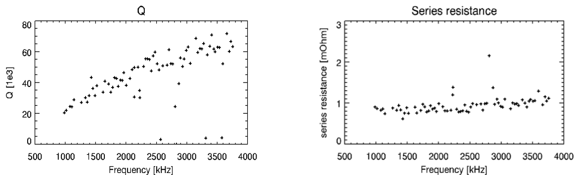
Figure 9a) Q values of the LC filters; b) parasitic resistance
