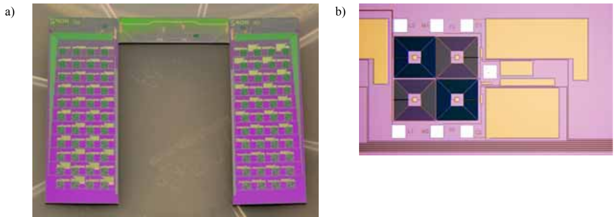
Figure 3 Two LC filters used for the 176 pixel FDM experiment.
