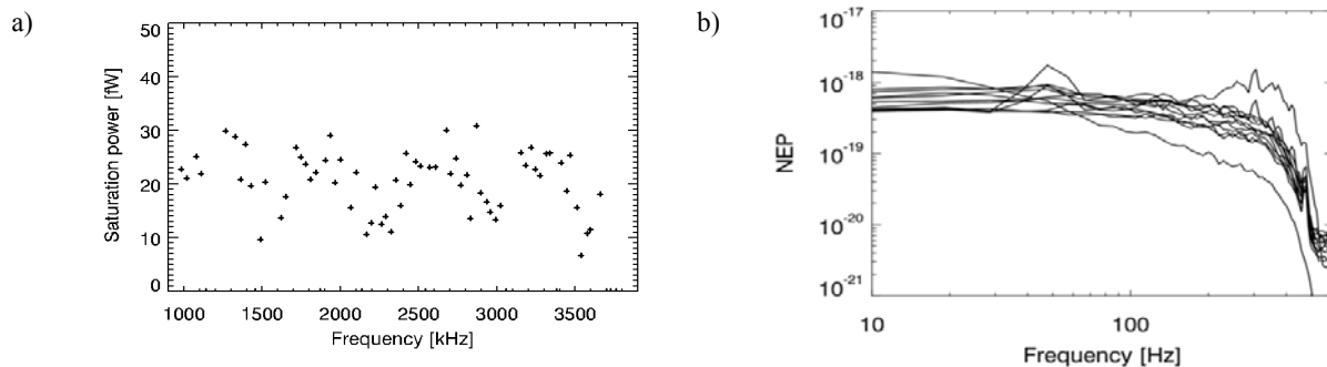
Figure 14 a) saturation power as function of resonance frequency and b) an example of the NEP of the TES bolometers.
