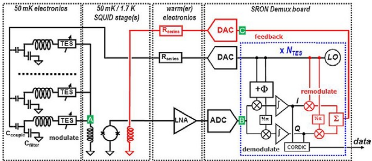
Figure 1. Schematic representation of the FDM bias and read out scheme.
