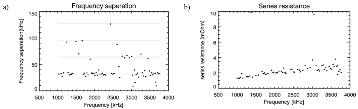
Figure 15. a) Frequency separation and; b) parasitic resistance of the right LC filter chip
