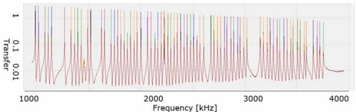
Figure 5 Example of a NWA scan via the bias line. Initially a rough scan use performed, to estimate the resonance frequencies, followed by individual detailed scans around the found frequencies.
