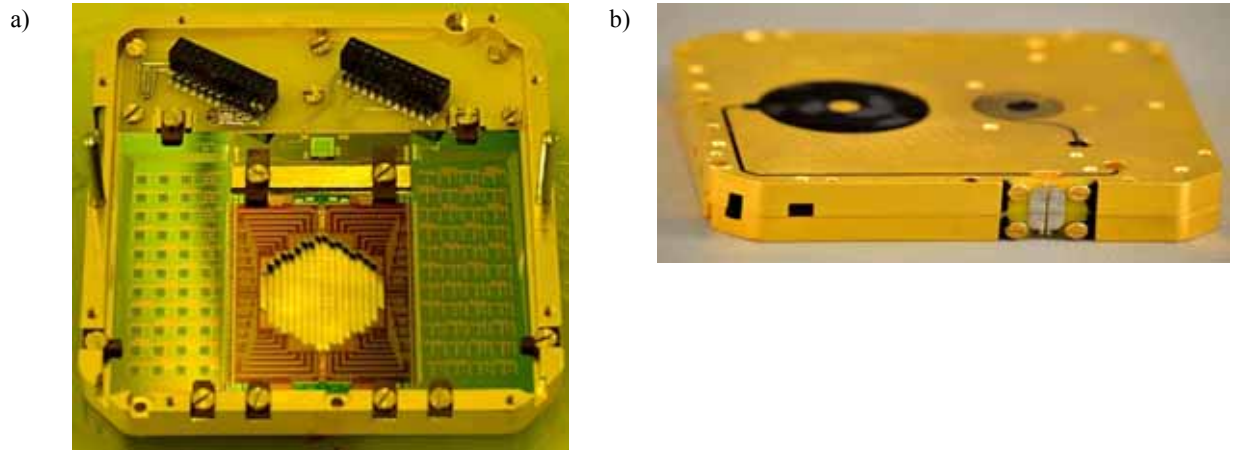
Figure 4 a) Assembled 176 pixel FDM experiment with SQUID fan out chip, LC filter chips and TES bolometer array; b) Same bracket but with the cover closed showing the integrated magnet and temperature sensor.
