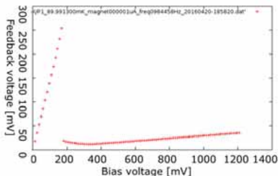
Figure 8. IV curve of one of the pixels to determine the setpoint in the transition of the TES
