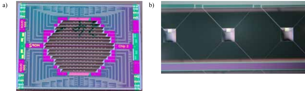
Figure 2 a) TES array containing 176 TES bolometers; b) a close up on some of the TES bolometers in the array.
