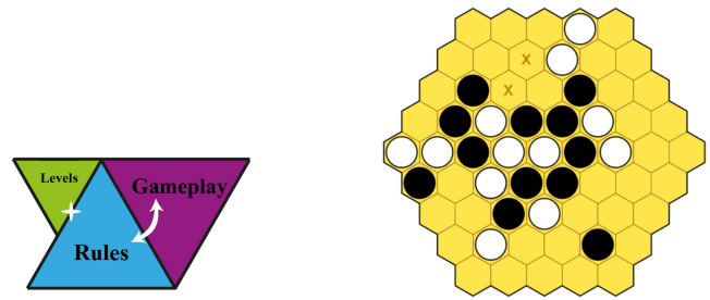
Fig. 15. Facet orchestration in Ludi, where the rules for black, white and neutral pieces are evolved alongside a board layout (i.e., a game level). Evaluation of the board and game piece rules is based on simulated playthroughs of two artificial agents using the same evolved policy based controllers. Screenshot of generated game Yavalath is from [30].
