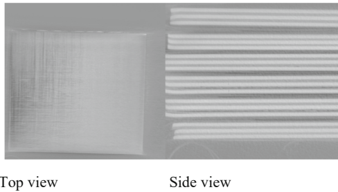
Fig. 10. X-ray CT image of a specimen with Loctite Frekote (mould release agent) inclusion.
