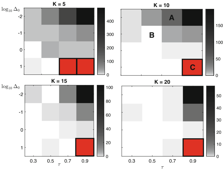
Fig. 5. Convergence time (from white to black) as a function of parameters \tau , \Delta_0 , and K . The red rectangles correspond to parameter values leading to wrong estimations.
