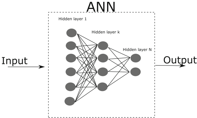
Fig. 7. ANN behavior
