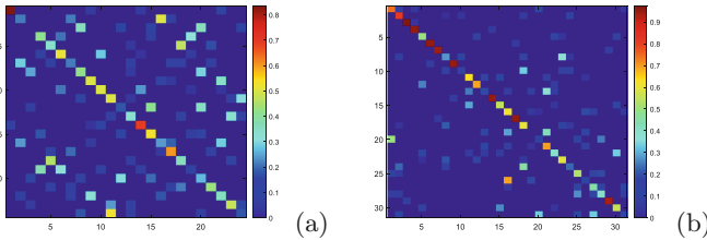
Fig. 4. Incremental learning. a) Corresponding TM to the situation model, b) TM after clustering the learnt Q-table.
