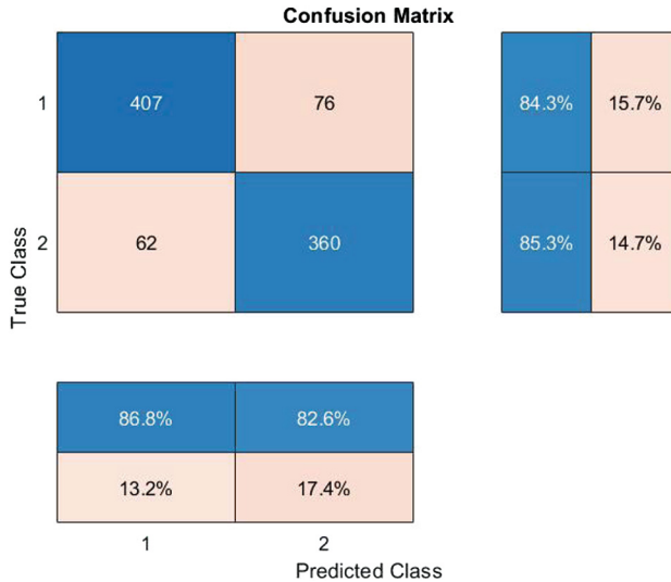
Fig. 9. Confusion Matrix in validation set for P_2
