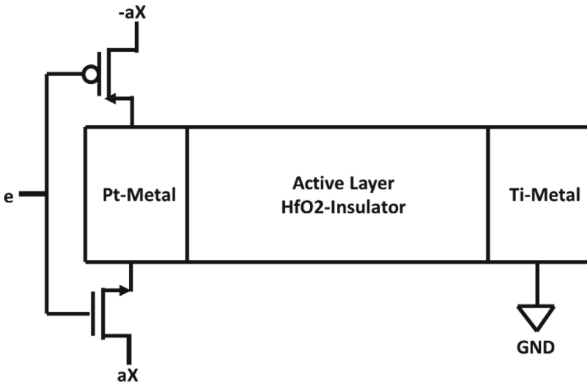
Fig. 2. 2T1M Synapse schematic in [10] used Pt-Hf-Ti memristor.
