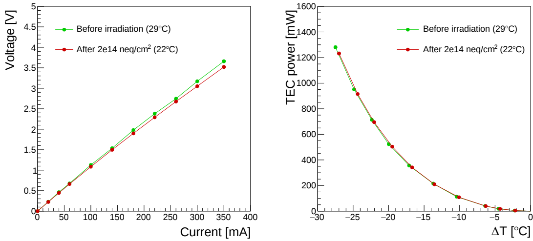
Figure 13. Measured voltage as a function of current (left panel) for four TECs connected in series on a SiPM package before (green) and after irradiation to 2 \times 10^{14} \text{ neq/cm}^2 (red) and corresponding TECs power as a function of the temperature gradient across the hot and cold surfaces (right panel).
