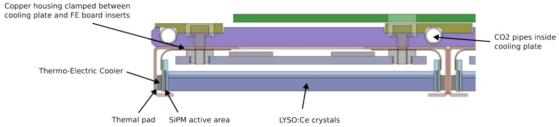
Figure 2. Transverse section of a BTL detector module attached to the cooling plate.
