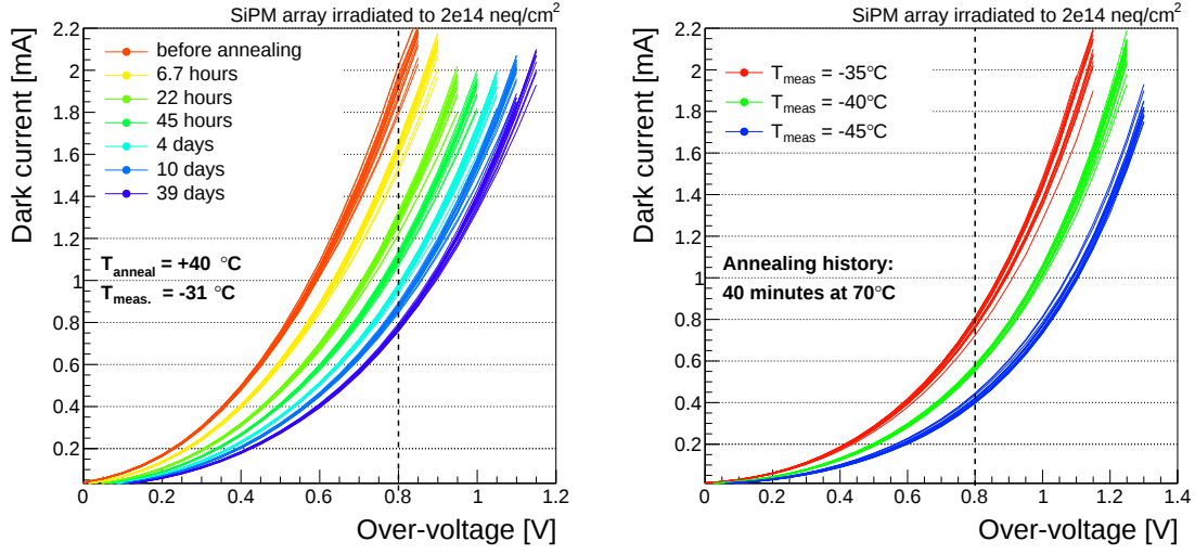
Figure 3. Left: dark current as a function of over-voltage measured at -31\text{ °C} across all 16 channels of a SiPM array irradiated to 2 \times 10^{14}\text{ neq/cm}^2 after different periods of annealing at 40\text{ °C} . Right: dark current of all 16 channels of a SiPM array irradiated to 2 \times 10^{14}\text{ neq/cm}^2 and annealed for 40 minutes at 70\text{ °C} , measured at different SiPM temperatures from -35\text{ °C} to -45\text{ °C} . The vertical dashed line at 0.8 V over-voltage serves the purpose to guide the eye to assess the impact of dark current reduction from annealing and lower operating temperature.
