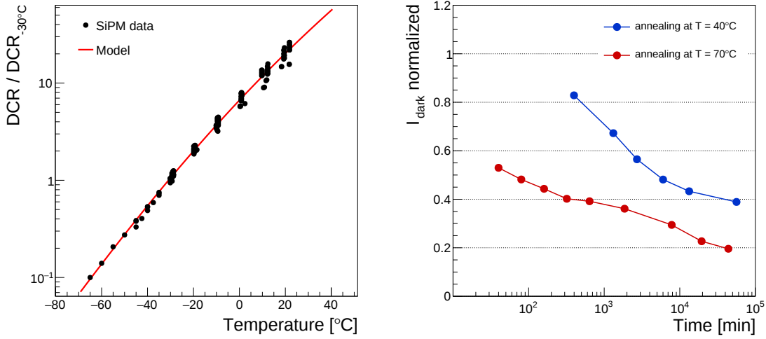
Figure 4. Left: dark count rate evaluated at 1 V over-voltage at a certain temperature T , relative to the dark count rate at T = -30^{\circ}\text{C} . Data points include results from a set of SiPMs irradiated to various fluences ( 1 \times 10^{13} , 5 \times 10^{13} , 2 \times 10^{14} and 3 \times 10^{14} \text{n}_{\text{eq}}/\text{cm}^2 ) interpolated with the parameterization described in eq. 2.1. Right: reduction of dark current over time due to thermal annealing at 40^{\circ}\text{C} and 70^{\circ}\text{C} normalized to the dark current measured after irradiation.
