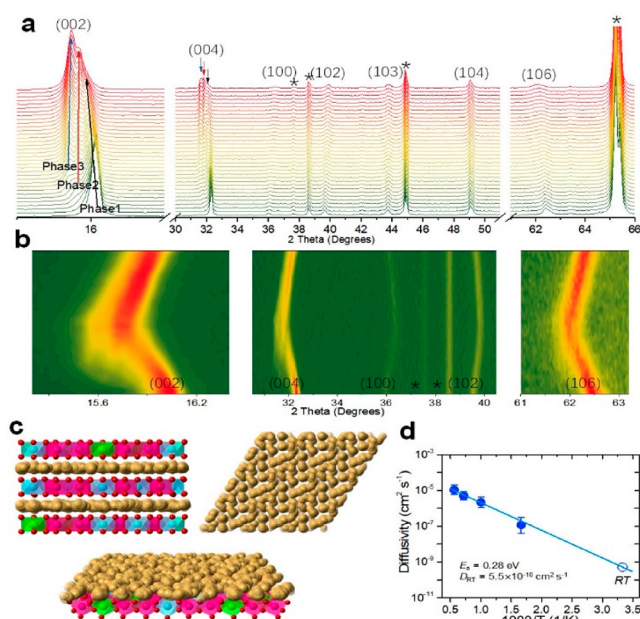
Figure 6. Structural evolution and Na + transport properties of this P2-type cathode. (a) In situ XRD patterns recorded at a rate of 0.05C charged to 4.60 V. The peaks marked by an asterisk originate from the casing of the in situ Swagelok cell. (b) In situ XRD patterns recorded at a high rate of 0.5C in the voltage range 2.0–4.0 V. (c) Na + migration pathway in the high Na-content P2-type oxide simulated at a temperature of \sim 1400 K over a period of 6 ps. The detailed views of Na + layers are given in the right and lower panels, where the yellow spheres indicate the trace of the Na + positions during MD simulations. (d) Arrhenius plot of diffusion coefficients resulting from the MD simulations, resulting in a Na + ion migration energy barrier of 0.28 eV.
