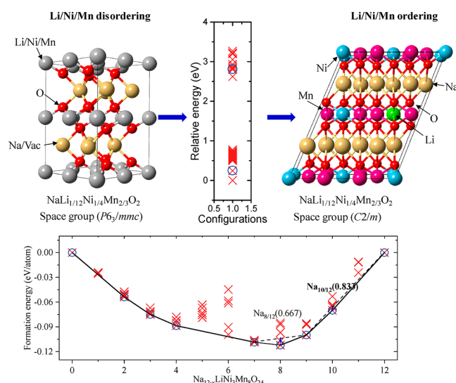
Figure 3. Determination of the Na/vacancy ordering and phase stability in convex hull. (a) Determination of the Li/Ni/Mn (dis)ordering in the system of \text{Na}_{12-x}\text{LiNi}_3\text{Mn}_8\text{O}_{24} . The detailed information on determination of the ground state structure and Li/Ni/Mn (dis)ordering in the system of \text{Na}_{12-x}\text{LiNi}_3\text{Mn}_8\text{O}_{24} is presented in Supporting discussion S1. (b) Phase stability in the \text{Na}_{12-x}\text{LiNi}_3\text{Mn}_8\text{O}_{24} - \text{LiNi}_3\text{Mn}_8\text{O}_{24} convex hull. The formation energy was calculated considering all possible Na and their vacancy configurations, and the potential structures with different Na contents were predicted in this study. Red crosses indicate the energies of different enumerated phases computed at the Na content. Blue circles are ground states, as they are part of the convex energy hull in solid line.
