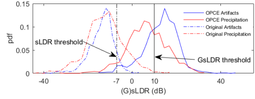
(a) (G)sLDR distribution of precipitation and artifacts
