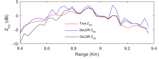
(b) Reflectivity comparison between different filters
