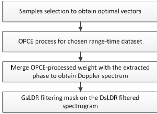
Fig. 1: Flow chart of OPCE-based clutter suppression method.
