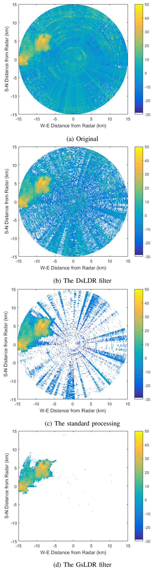
Fig. 4: Radar PPI after different processing.
