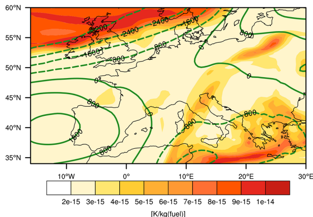
Figure 2. Water vapor aCCF at a pressure level of 250 hPa over Europe at 12:00 UTC on 15 June 2018. Units are given in [\text{K kg}(\text{fuel})^{-1}] . Overlaid green lines indicate positive (solid line) and negative (dashed line) geopotential height anomalies (in \text{m}^2 \text{ s}^{-2} ).
