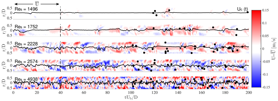
Figure 3.4: Streamwise velocity patterns ( u_x' ) as a function of time for various Reynolds numbers. The concentration for this case is \phi = 0.05\% . Particles are shown only for the second part of the time series ( tU_b/D > 100 ).
