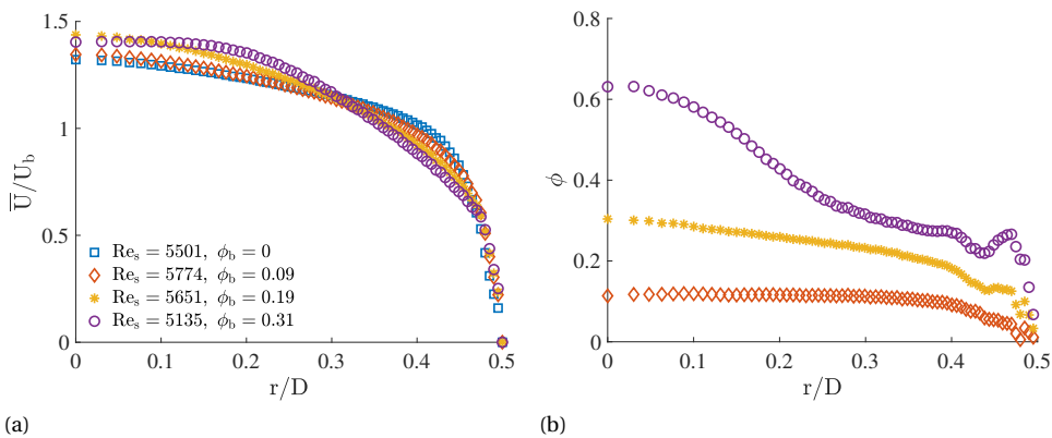
Figure 5.4: Velocity (a) and concentration profiles (b) for constant suspension Reynolds number, Re_s = 5000 , and increasing volume fraction.
