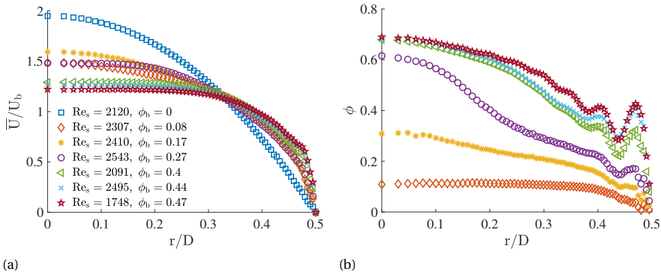
Figure 5.3: Velocity (a) and concentration profiles (b) for constant suspension Reynolds number, Re_s = 2000 , and increasing volume fraction. The exact suspension Reynolds numbers and bulk volume fractions are shown in the legend in (a).
