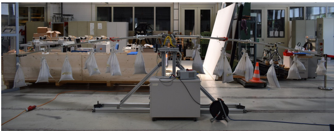
Figure 18: Airworthiness test – stand-stand (above) and loaded wings (below)
