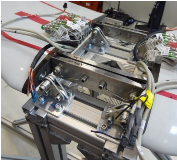
a.) Wing clamped to the test stand
