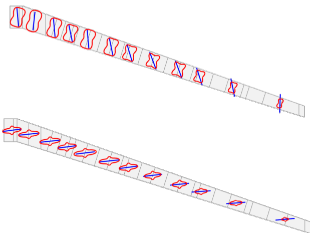
Figure 5: Polar distribution of in-plane stiffness term A_{11} in the reference design (top) and tailored design (bottom), for the upper skin
