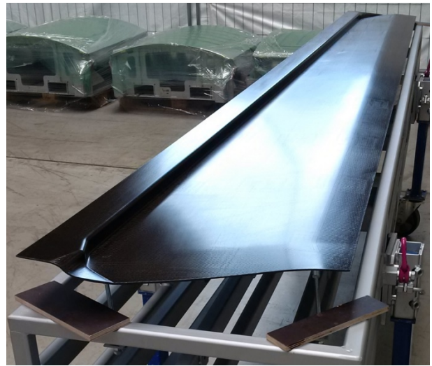
a.) CFRP mould for the wing skin
