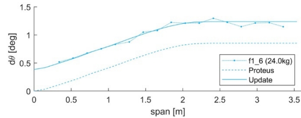
Figure 14: Initial and updated PROTEUS model vs. experimental results – span-wise twist
