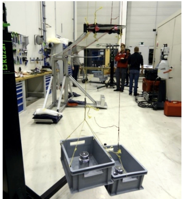
b.) Static load application
