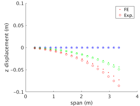
Figure 15: Initial FE model vs. experimental results – span-wise displacement (different colours representing the different load-magnitudes)
