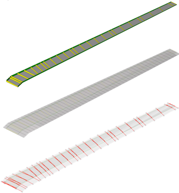
Figure 3: NASTRAN models used in Step 2 of the optimization workflow – structural FE model, aerodynamic DLM model, coupled aeroelastic splining model
