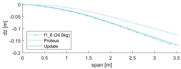
Figure 13: Initial and updated PROTEUS model vs. experimental results – span-wise displacement
