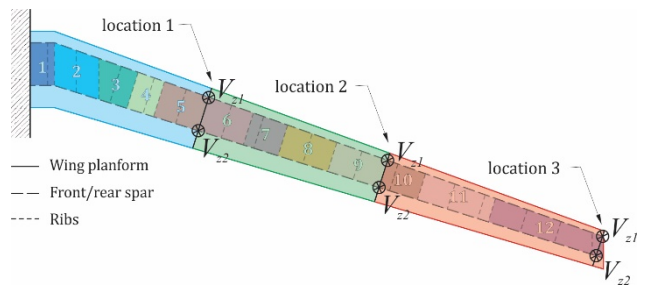
Figure 11: Load application points
