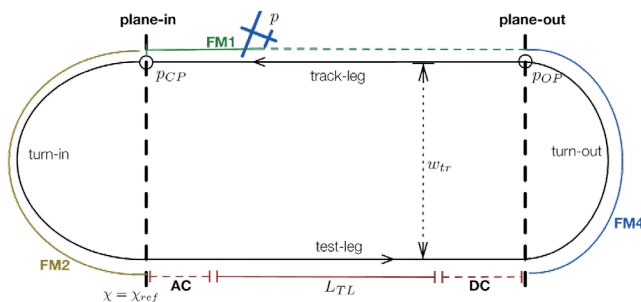
Figure 20: Test-leg for the FLEXOP UAV
