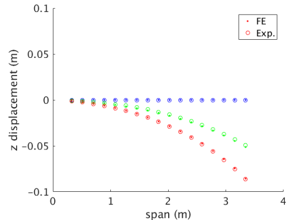
Figure 16: Updated FE model vs. experimental results – span-wise displacement (different colours representing the different load-magnitudes)
