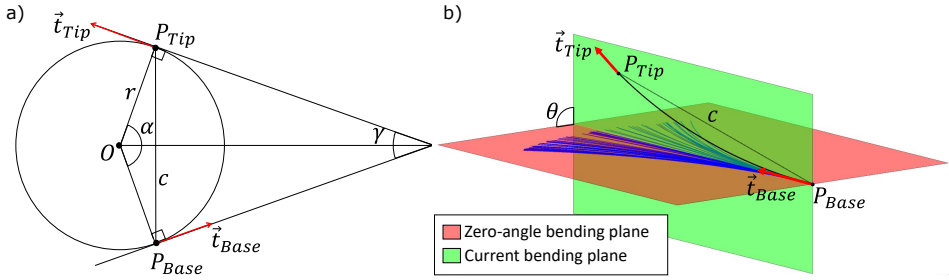
Figure 4.4: The calculation of the curvature and the angle of the bending plane, which are explained in Section 4.3.2: (a) curvature calculation; (b) \theta is the angle between the zero-angle bending plane and the current bending plane.
