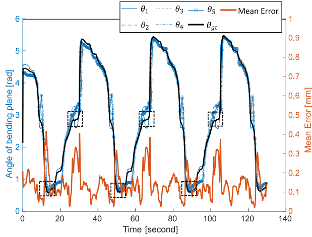
Figure 4.13: The estimated angles of the bending plane of each grating (blue), ground truth angle of the bending plane (black) and mean error (orange) of lissajous (1) experiment are plotted over the time. Transition regions where there are increases in mean error are marked with dashed square.
