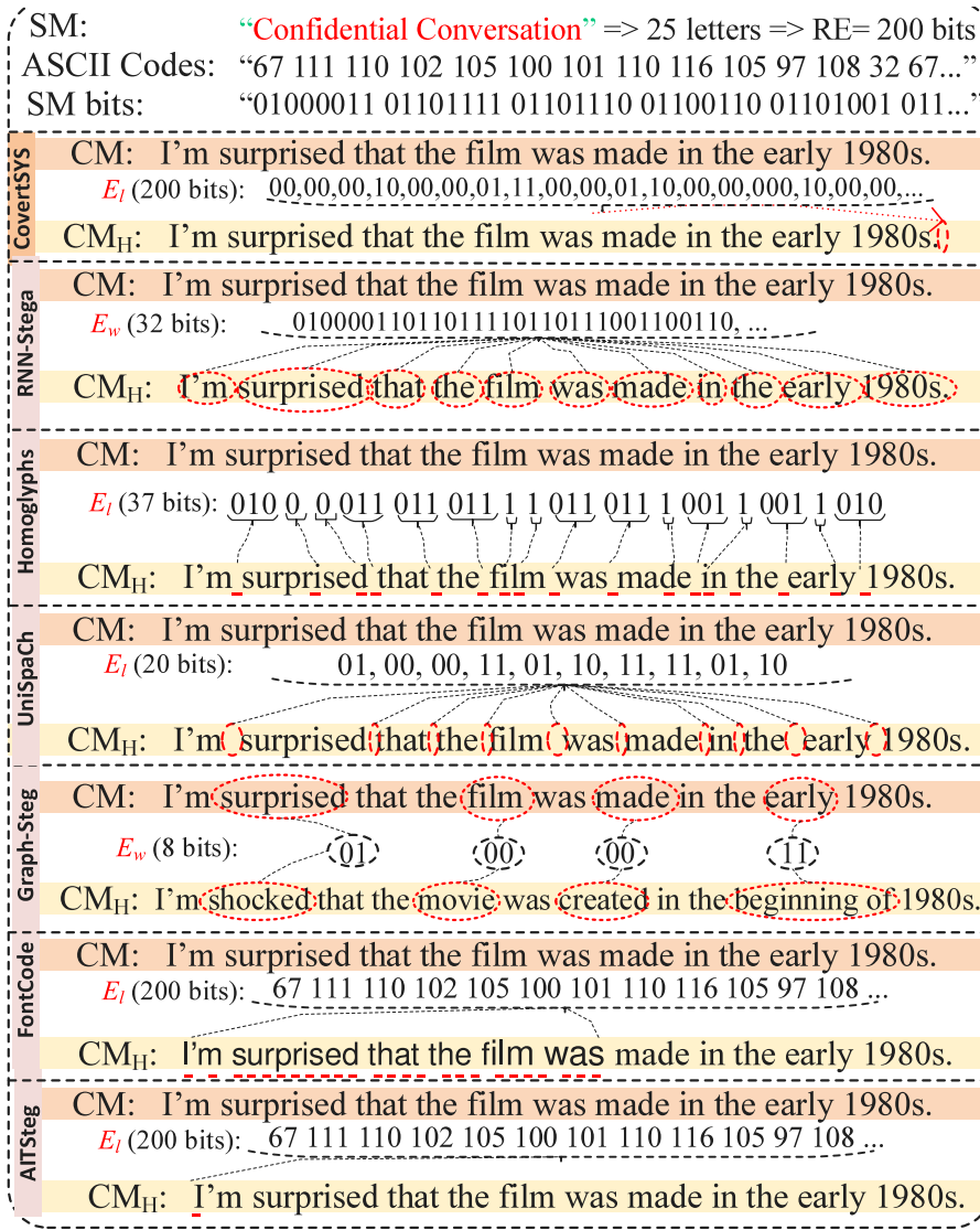
Fig. 4. An illustration of embedded spots of aforementioned techniques on the same SM and CM example.
