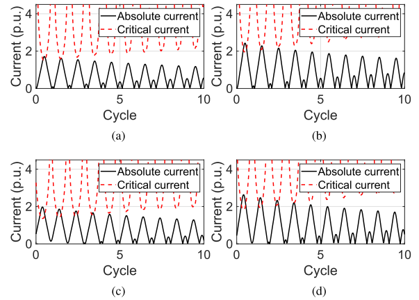
Fig. 8. Short-circuit currents in Phase A (in absolute value) compared with critical currents for the ISDW design. (a) PF = 0.7 , no-load. (b) PF = 0.8 , no-load. (c) PF = 0.7 , rated-load. (d) PF = 0.8 , rated-load.
