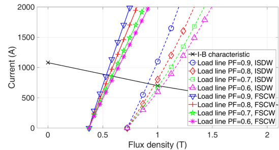
Fig. 3. Load lines and I-B characteristic for determining critical currents of the MgB_2 winding for generator designs with different power factors.
