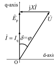
Fig. 2. Phasor diagram of a generator with zero d-axis current control.
