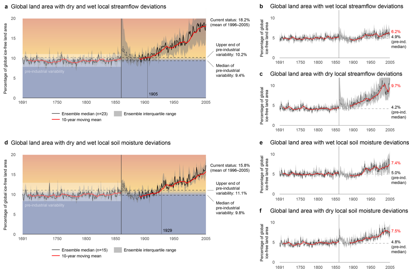
Extended Data Fig. 1 | Percentage of global ice-free land area with local deviations, separately for summed, wet and dry deviations. Panels show the percentage of land area with local streamflow (a–c) and soil moisture (d–f) deviations, dry and wet local deviations summed (a, d), and for wet (b, e) and dry (c, f) local deviations separately. Shown is the annual percentage, which is computed as an average of monthly percentages. The annotated years mark the 10-year moving (trailing) mean transgressing the upper end of pre-industrial variability (95th percentile of the pre-industrial percentage of land area with local deviations; Fig. 1d). The ensemble median and interquartile range are computed
