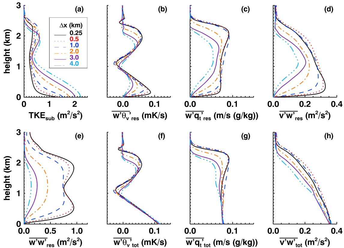
Figure 17. Reference case results of horizontal mean values of (a) the subgrid TKE, the resolved vertical fluxes of (b) \theta_v , (c) q_t , and (d) v , (e) the resolved vertical wind variance \overline{w'w'} , and the total vertical turbulent fluxes of (f) \theta_v , (g) q_t , (h) and v at t = 12 hr. The results represent 10-min-averaged values obtained from DALES with different meshes \Delta x of 0.25, 0.5, 1, 2, 3, and 4 km. The line styles are according to the legend. TKE = turbulent kinetic energy.
