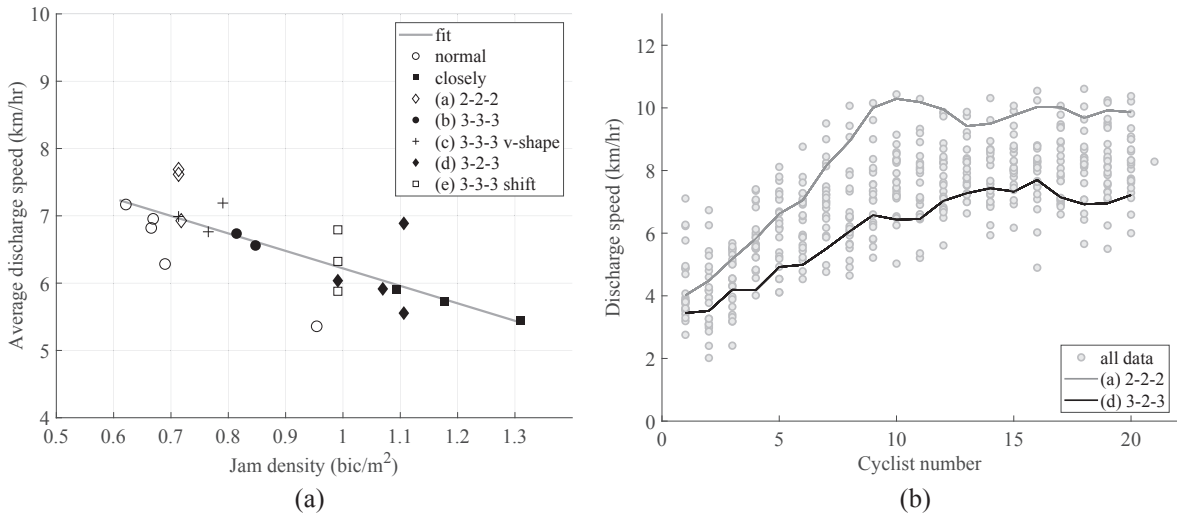
Fig. 8. Results of the experiment, with (a) the queue discharge rate and (b) the average speed that cyclists had while passing the stop line.
