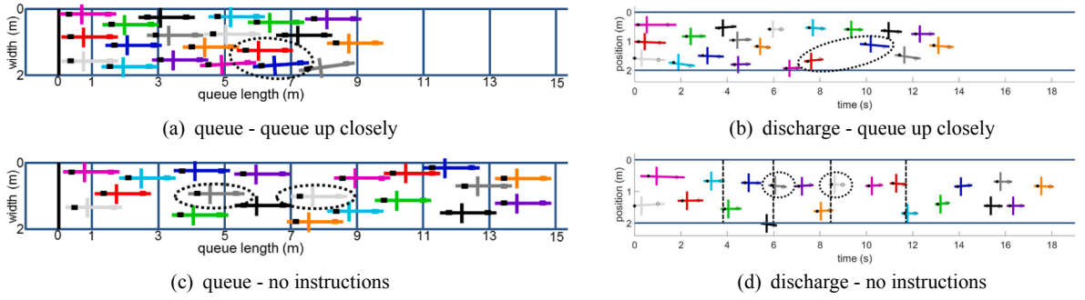
Fig. 10. Observed queue and discharge configurations.
