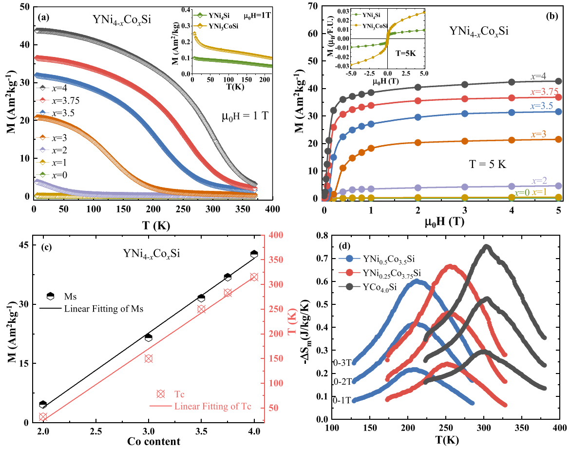
Fig. 2. (a) Magnetization as a function of temperature in an applied field of 1 T and (b) magnetization as a function of magnetic field at 5 K of YNi 4-x Co x Si ( x = 0-4 ) (inset shows an enlargement of the weak magnetisation curves for x = 0-1 ). (c) Values of T_c and M_s for YNi 4-x Co x Si ( x = 0-4 ) as a function of the Co content. (d) Isothermal entropy change -\Delta S_m obtained from the magnetisation M(T) upon heating in a field change of 1, 2 and 3 T.
