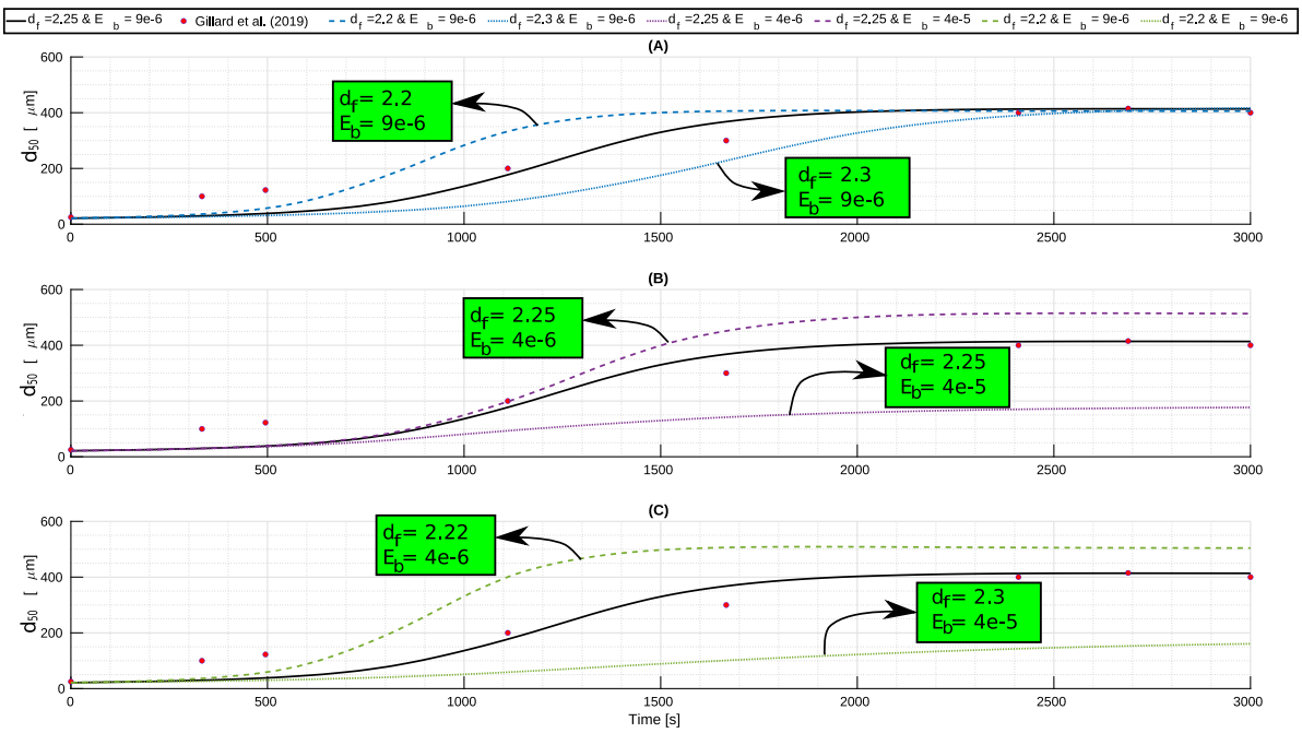
Fig. 5. Calibration process in case of 105 mg/l mass concentration and 2.4 \text{ s}^{-1} shear rate. All 3 figures show the development of d_{50} over time. (A) represents the sensitivity of the fractal dimension d_f on the numerical results, where the breakage coefficient E_b = 9 \times 10^{-6} is constant. (B) represents the sensitivity of the breakage coefficient, where the d_f = 2.25 is constant. (C) represents the sensitivity of both parameters d_f and E_b on the development of d_{50} .
