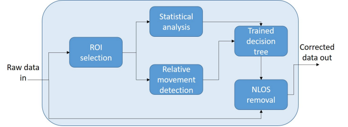
Fig. 13: Block diagram of the algorithm implemented.
