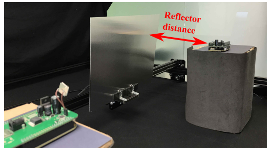
Fig. 2: Testbed.
