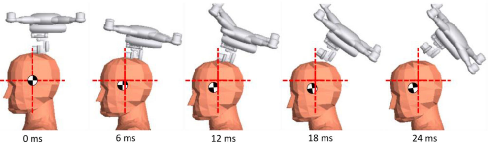
Figure 5. Comparison of impact sequences between the Hybrid III and the human body for \theta = 90^\circ (vertical drop) and \psi = 0^\circ, 90^\circ and 180^\circ at 196 J impact energy (equivalent to 18 m/s impact velocity).
