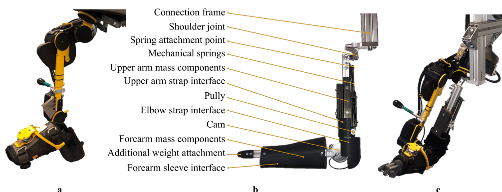
Figure 1. Picture of the (a) DAROR exoskeleton, the (b) dummy arm design with its components, and (c) the dummy arm placed inside the DAROR exoskeleton.
