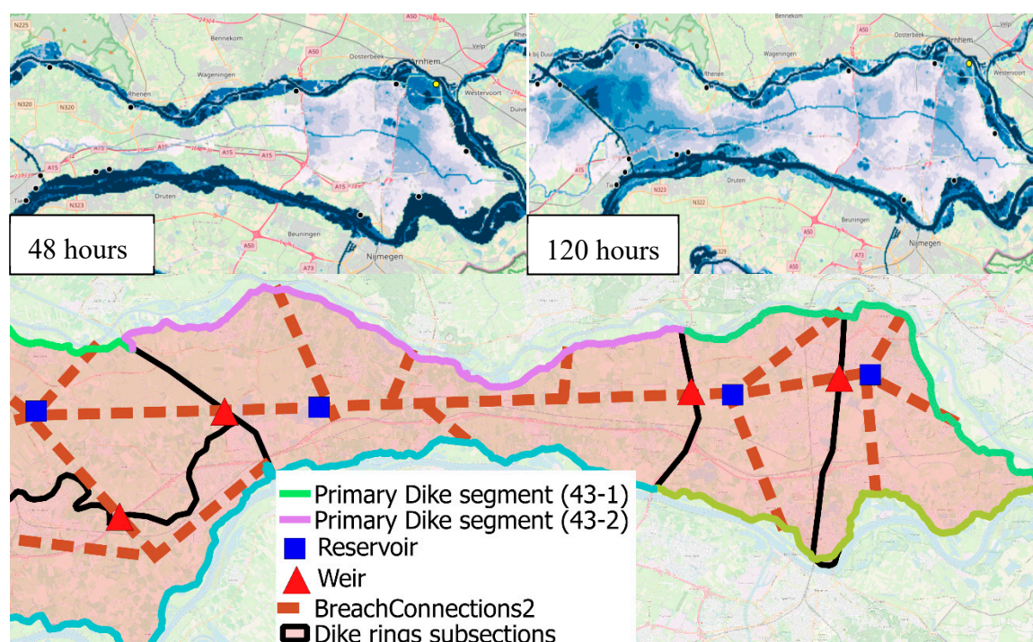
Figure 2. Top panels: Flooding from the Lek to dike ring 43 over time. Bottom panel: resulting delineation and schematisation of dike ring 43 based on flood simulations.
