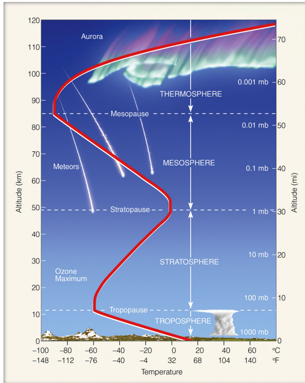
Figure 2.1: The structure of the atmosphere and the variation of air temperature, taken from https://ghsearth.weebly.com/atmosphere.html (last accessed on 23rd February 2024).
