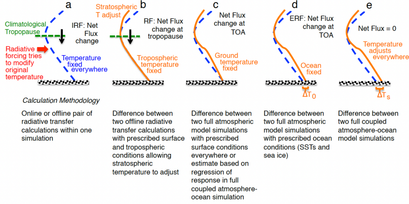
Figure 2.3: Comparing various definitions for RF: (a) instantaneous RF (b) stratospheric adjusted RF, (c) flux change when the surface temperature is fixed, enabling a calculation of ERF, (d) ERF allowing atmosphere and land temperature to adjust while keeping ocean conditions such as Sea Surface Temperature (SST) and sea ice fixed, and (e) the equilibrium response to the perturbation. The methodology for calculating each RF is highlighted. \Delta T_0 represents land temperature response while \Delta T_s represents the temperature response of Earth's entire surface. This figure is taken from IPCC [8], which is adapted from Hansen [50].
