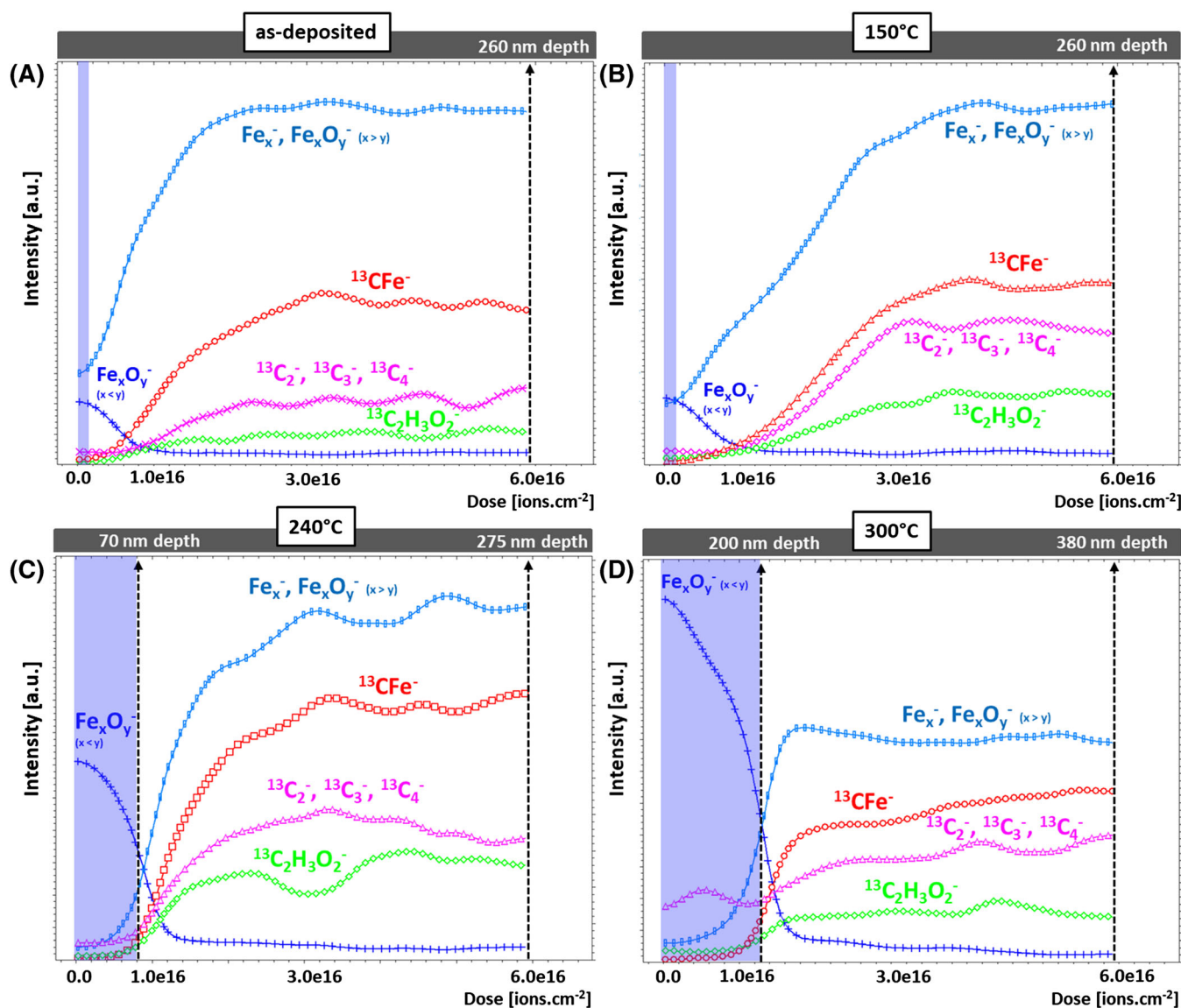
FIGURE 4 ToF-SIMS depth profiles obtained with a 20 keV Ar 1200 + sputter source for (A) the as-deposited Fe- 13 C coating and for the Fe- 13 C coatings annealed at (B) 150°C, (C) 240°C, and (D) 300°C. Depths shown in the profiles are derived from AFM line scans across the sputter craters (Figure S4). Native iron oxide layers (for as-deposited and 150°C) and thermal iron oxide layers (for 240°C and 300°C) are shaded in blue.
