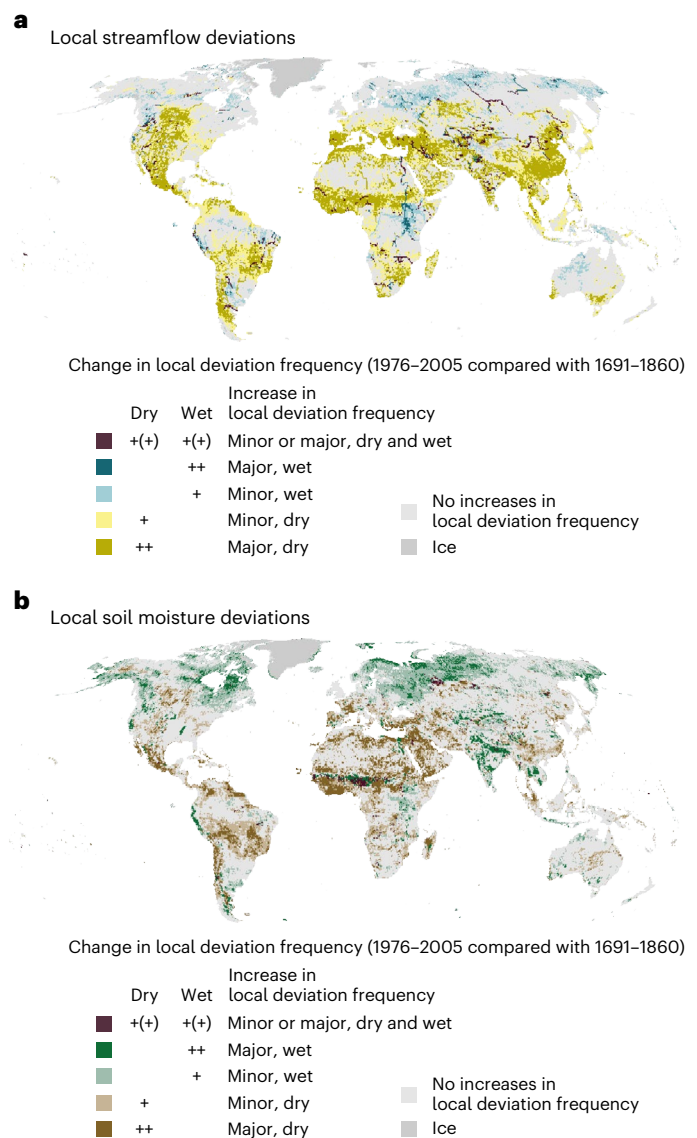
Fig. 3 | Statistically significant increases in dry and wet local deviation frequency. a,b, For streamflow (a) and soil moisture (b), changes in the frequency of local deviations are computed by comparing the ensemble median frequency of local deviations during 1976–2005 against 1691–1860, and significance of change is tested at a 95% confidence level ( P = 0.05 ) with R package stats function prop.test 96 (one-sided test). Colours denoted with ‘+’ indicate statistically significant increases with magnitude \leq 5 p.p. (minor), whereas colours denoted with ‘++’ indicate statistically significant increases with magnitude > 5 p.p. (major). Colours denoted with ‘+(+)’ pool together any statistically significant increase (minor or major).
