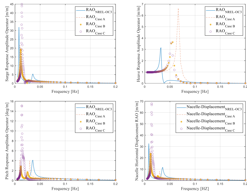
Figure 5. Surge, heave, pitch and nacelle displacement RAO.
