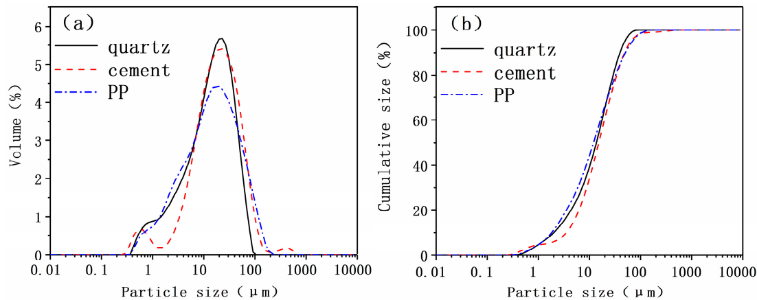
Figure 1. Volume distribution of particle size (a) and cumulative distribution of particle size (b) of quartz, cement, and ceramic polishing powder (PP).
