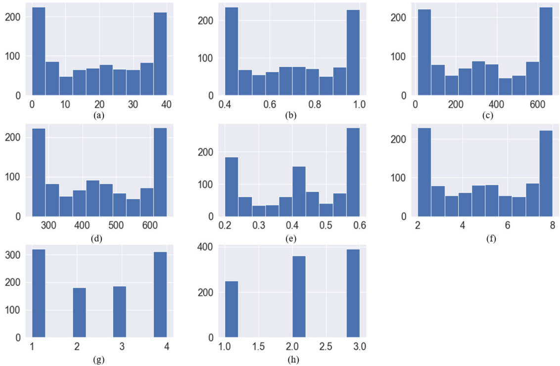
FIGURE 16 AEL sampling results of uncertainty-based query: (a) temperature (°C); (b) relative humidity (%); (c) TIME of curing (hours); (d) cement amount (kg/m 3 ); (e) w/c ratio; (f) a/c ratio; (g) aggregate type; (h) cement type. The Y-axis presents the number of samples.
