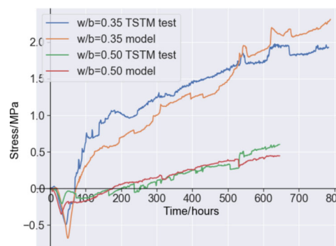
FIGURE 11 Comparison between TSTM tests and modeling results
