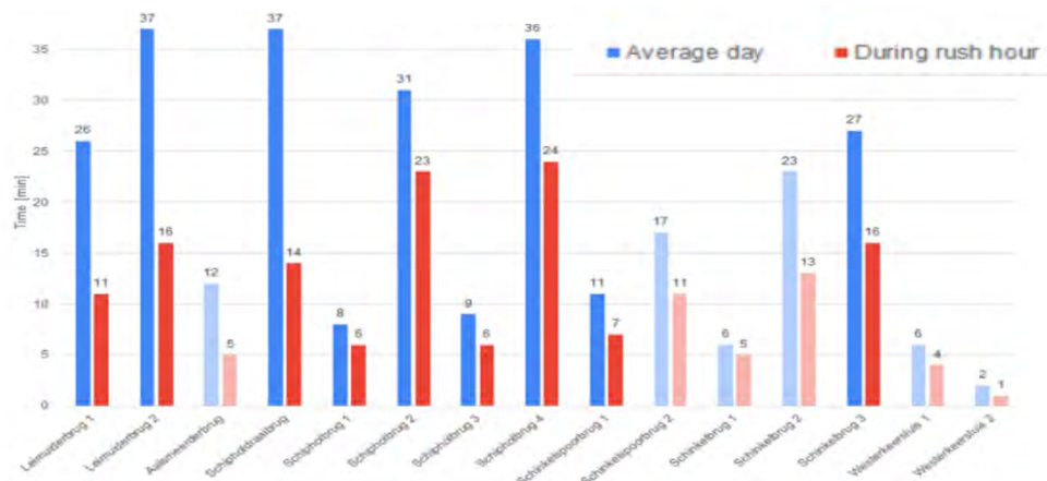
Fig.3: Maximum bridge opening times on an average day and at rush hour
