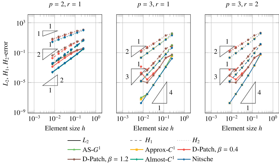
Fig. 9. Errors for the AS- G^1 , Approx. C^1 , D-Patch and Almost- C^1 construction for the biharmonic problem on the domain in Fig. 8. The L_2 , H_1 and H_2 errors with respect to the analytical solution are plotted with different line styles in the top row. Furthermore, all results are plotted against the element size h and the expected convergence rates are given by the triangles.
