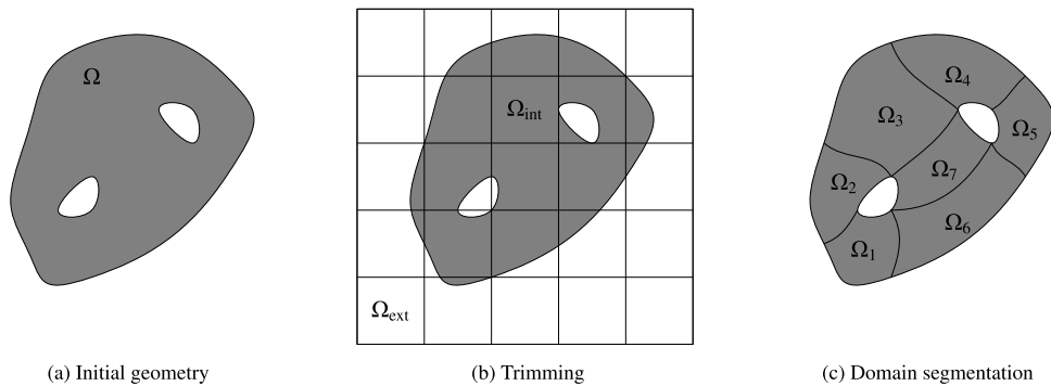
Fig. 3. Given an initial geometry \Omega (a), trimming (b) uses the curves of the boundary of the original geometry to define the interior domain \Omega_{\text{int}} and the exterior domain \Omega_{\text{ext}} . An alternative approach for modelling the domain is to use domain segmentation (c). Here, the domain is decomposed into several patches \Omega_i which together define the full domain \Omega .
