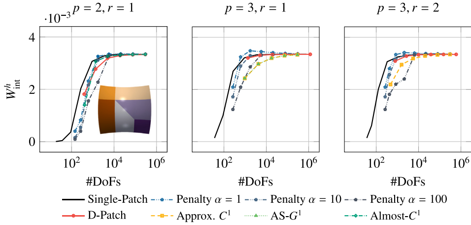
Fig. 12. Bending energy norm W_{\text{int}}^h = \frac{1}{2} \mathbf{u}_h^T \mathbf{K}_h \mathbf{u}_h for the hyperboloid geometry from Fig. 10 with a patch segmentation as in Fig. 8. The results are presented for different combinations of the degree p and regularity r for all unstructured spline constructions. In addition, the results for a penalty method with parameter \alpha \in \{1, 10, 100\} are provided for comparison.
