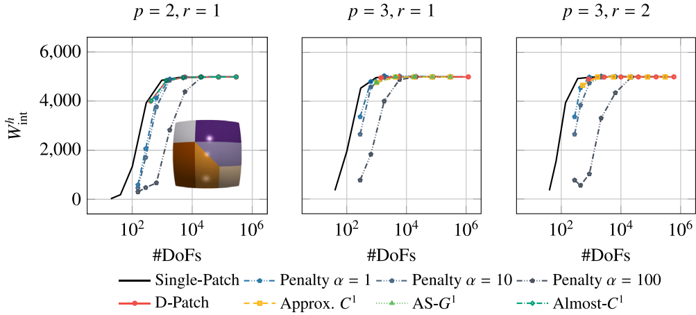
Fig. 13. Bending energy norm W_{\text{int}}^h = \frac{1}{2} \mathbf{u}_h^T \mathbf{K}_h \mathbf{u}_h for the paraboloid geometry from Fig. 11 with a patch segmentation as in Fig. 8. The results are presented for different combinations of the degree p and regularity r for all unstructured spline constructions. In addition, the results for a penalty method with parameter \alpha \in \{1, 10, 100\} are provided for comparison.
