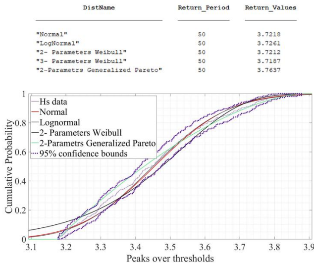
Figure 6: CUMULATIVE PROBABILITY AND DIFFERENT FITTING DISTRIBUTION FOR PKS ALONG WITH RETURN PERIOD OF 50 YEARS AND CORRESPONDING RETURN VALUE FOR PKS
