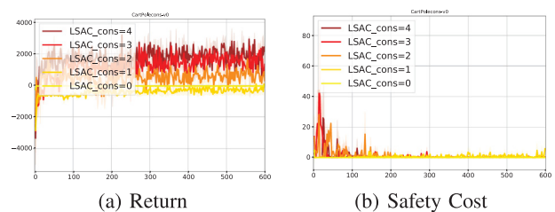
Fig. 7. The average return and constraint function of LSAC in Cartpole-Safe with different constraints \bar{x} .
