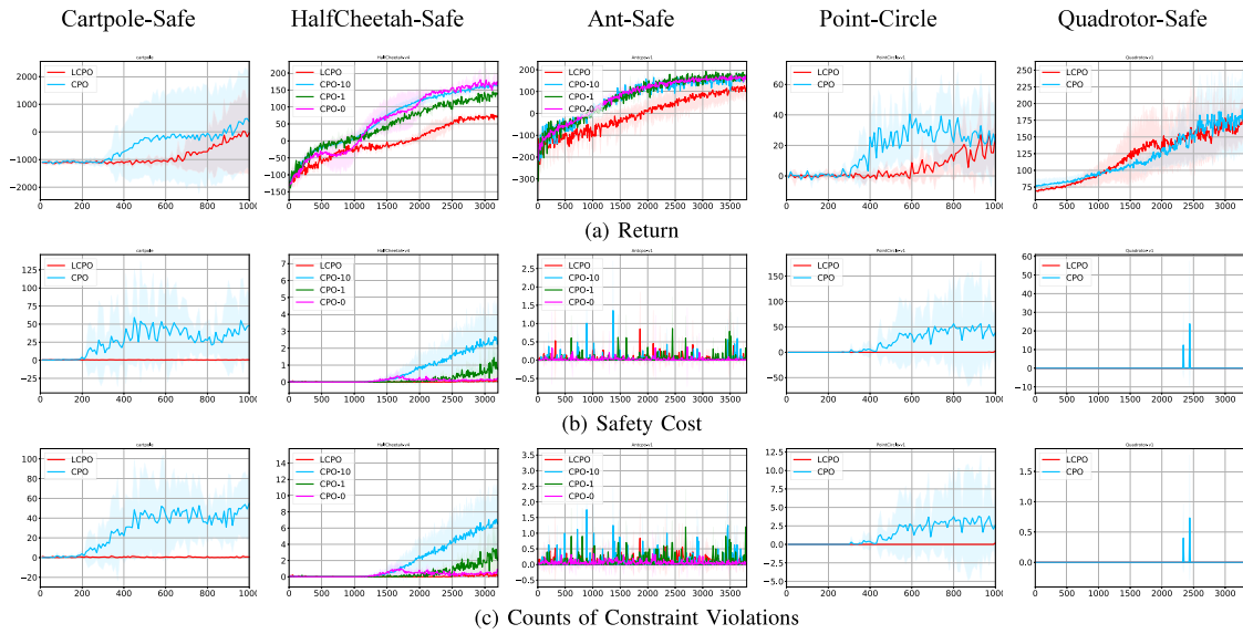
Fig. 5. The average performance of CPO and LCPO, where the shaded areas show the 1-SD confidence intervals over 5 random seeds. The X-axis indicates the total time steps in thousands. The return (a), safety cost (b), and counts on constraint violations (c) are shown in each row respectively.
