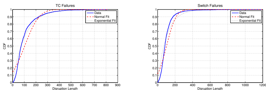
(a) Distribution of TC Disruption Length.
