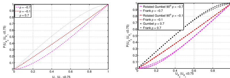
(a) Three different U_2 | U_1 \leq 0.75 from three normal copulas. (b) Six different U_2 | U_1 \leq 0.75 from three Frank copulas and three Gumbel copulas.
