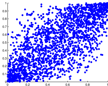
(a) Scatter plot of data sampled from a normal copula in Figure 1.9(a).
