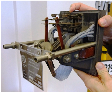
(b) A B2 Vane Relay.
