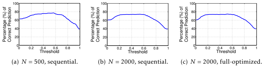
Figure 2.10: Proportion of correct prediction as a function of threshold value.
