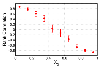
(a) Rank correlations.
