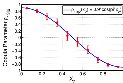
(b) Copula parameters and the function of \rho_{13|2}(x_2) .
