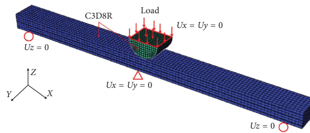
FIGURE 7: Finite element model for three-point bending.
