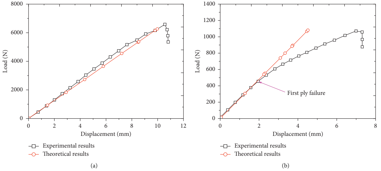
FIGURE 3: Load-displacement curve. (a) Longitudinal. (b) Transverse.
