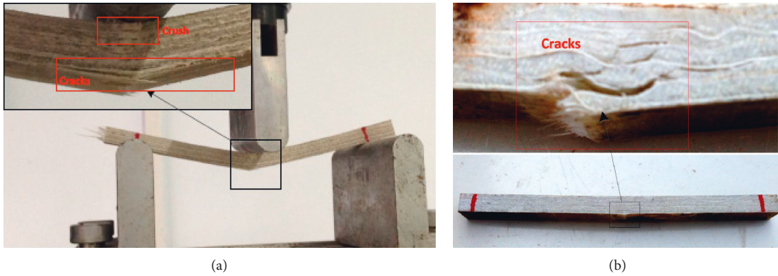
FIGURE 4: Failure modes. (a) Longitudinal. (b) Transverse.
