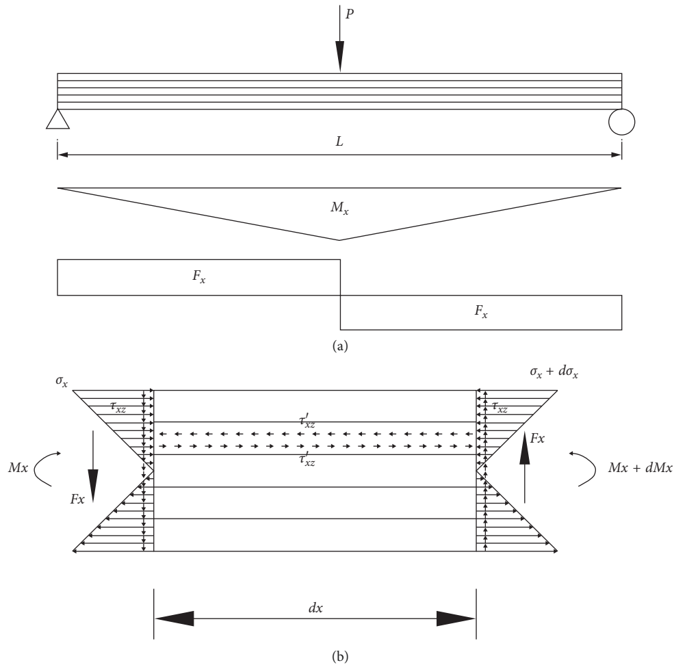
FIGURE 5: Loads and flexural stress distributions of three-point loading laminated beam. (a) Bending moment and shear force distribution. (b) Stress distribution of infinitesimal section.
