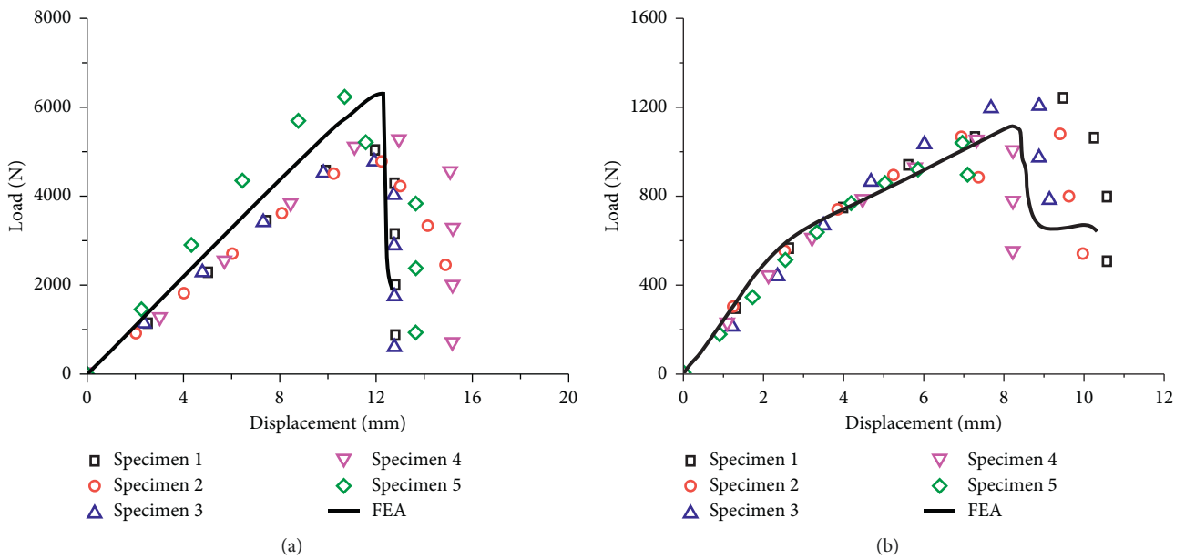
FIGURE 8: A comparison between numerical and experimental load-displacement relationship. (a) Longitudinal. (b) Transverse.
