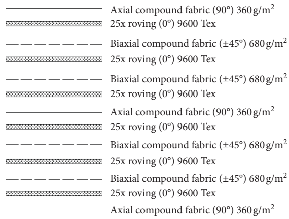
FIGURE 1: Laminate layup.
