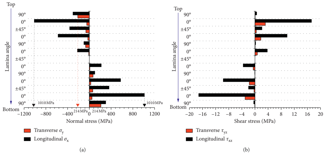
FIGURE 6: Laminate stress distribution along thickness direction. (a) Normal stress. (b) Shear stress.
