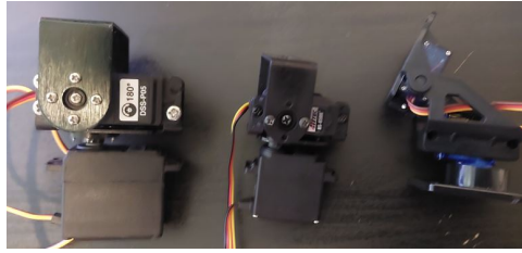
Figure 2.9: Pan/tilt platforms tested. Left: DF05BB; Middle: RB-Lyn-316; Right: ROB-1439
