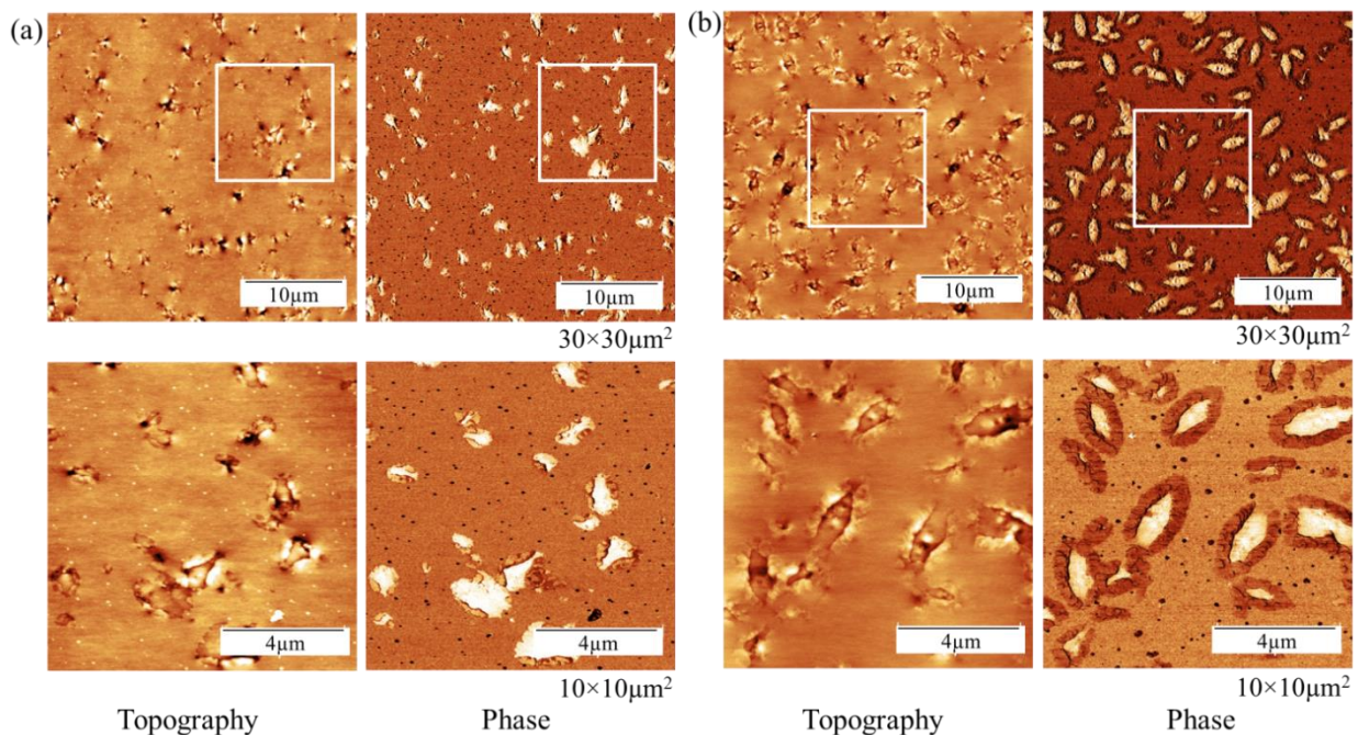
Figure 6: AFM topography and phase images of bitumen microstructure, captured at 25 °C after cooling from 90 °C to 25 °C. 30×30 µm 2 overview and 10×10 µm 2 zoomed in images of a) 70/100 and (b) 160/220.
