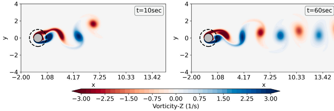
Fig. 14. Vorticity field for the case of the rotating cylinder at Re = 200 and \alpha = 0.5 . The numerical boundary is represented with a black dashed circle line.
