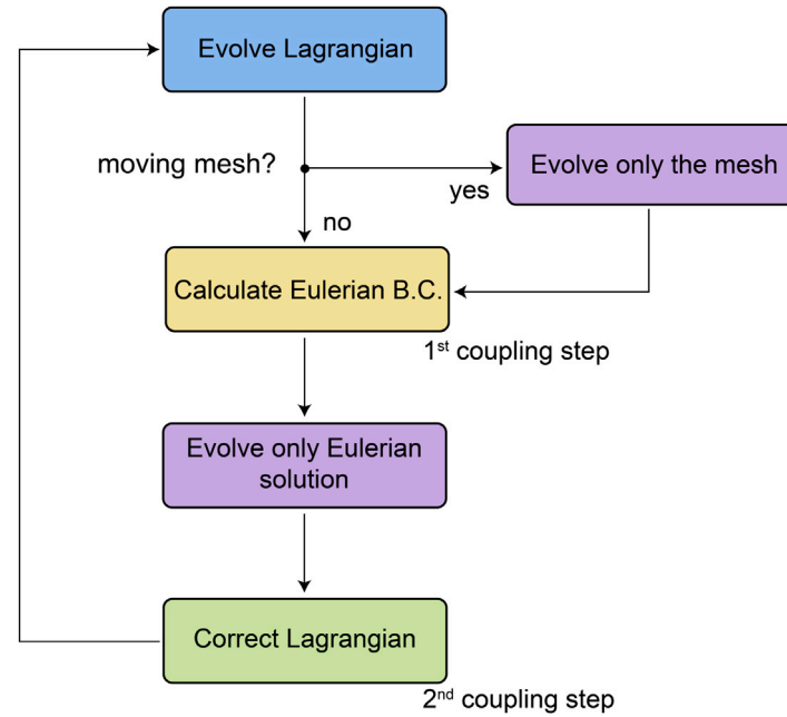
Fig. 3. The flowchart of the hybrid solver, including the mesh update, assumes that both solvers are at time t_n , and their solutions are correct. The first step is to evolve the Lagrangian solver to t_{n+1} . Then, if the body is moving, the mesh is moved; otherwise, the calculation of the Eulerian boundary conditions takes place directly. Subsequently, the Eulerian solution is evolved to t_{n+1} , and finally, the Lagrangian solver is corrected inside the interpolation region.
