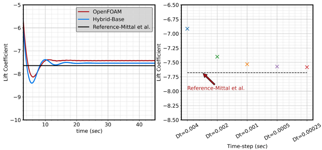
Fig. 15. On the left is the lift coefficient over time for the hybrid case, the OpenFOAM case, and the Ref. [24]. The time step convergence test for the lift coefficient is on the right compared to the Ref. [24].
