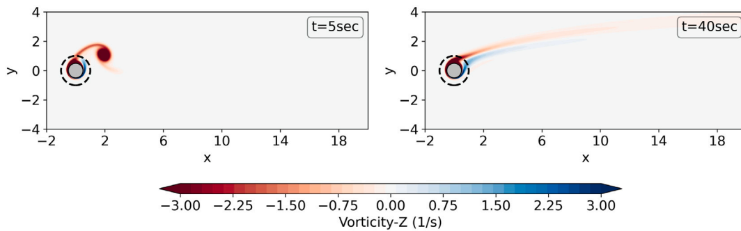
Fig. 16. Vorticity field for the case of the rotating cylinder at Re = 200 and \alpha = 2.5 . The numerical boundary is represented with a black dashed circle line.
