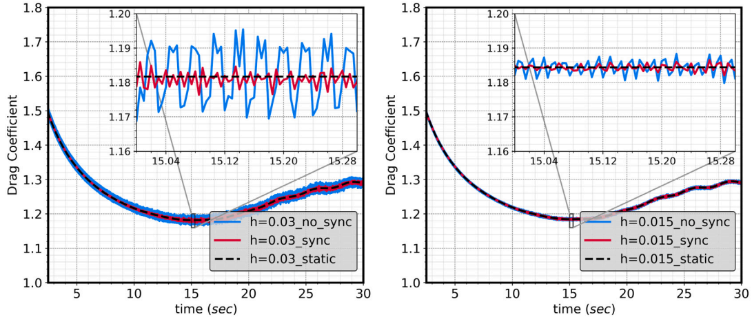
Fig. 8. Drag coefficient over time for different test cases of the traveling cylinder at Re = 100 , that demonstrate the alleviation of the high-frequency oscillations on the body forces.
