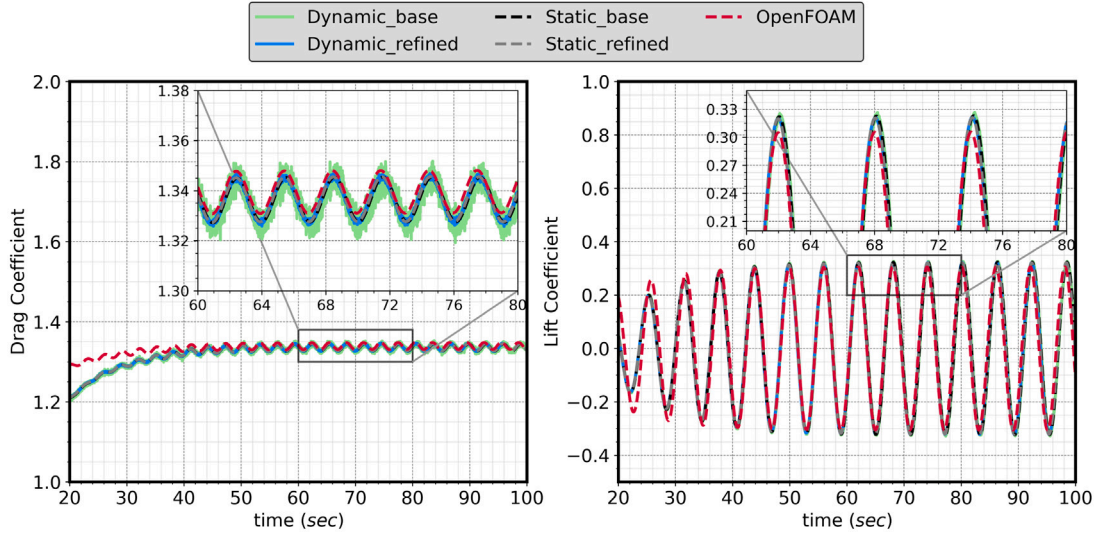
Fig. 10. Lift and drag coefficient over time for the case of the traveling cylinder at Re = 100 .
