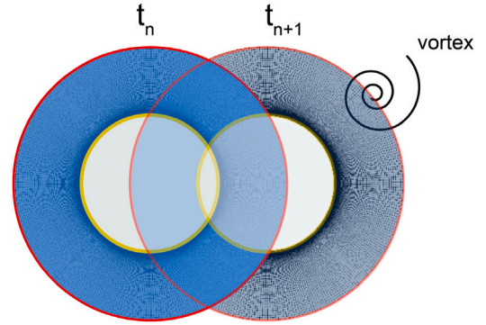
Fig. 2. A vortex that inserts in the Eulerian subdomain when the Eulerian mesh moves towards it. This is just a graphical representation for clarifying purposes since the body cannot cover this distance in one time step.
