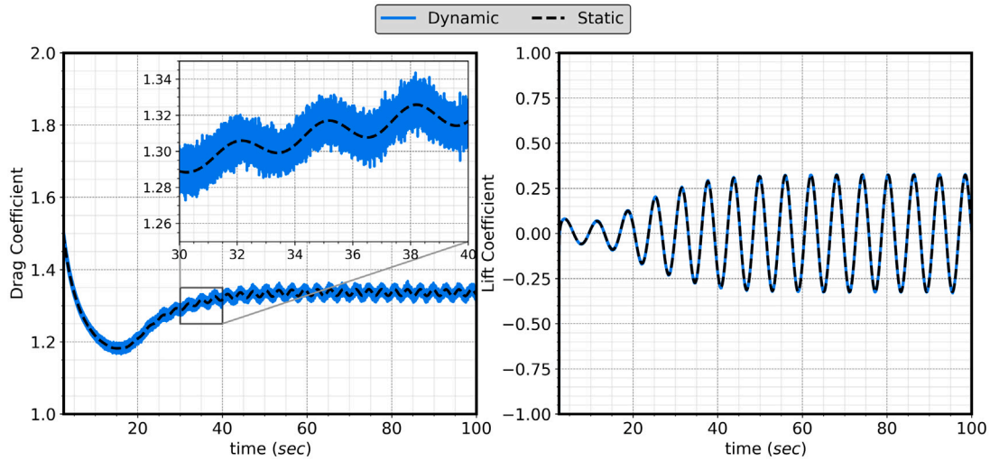
Fig. 6. Lift and drag coefficients over time for the case of the static and traveling cylinder at Re = 100 , with the base Eulerian mesh and particle spacing h = 0.03 m.
