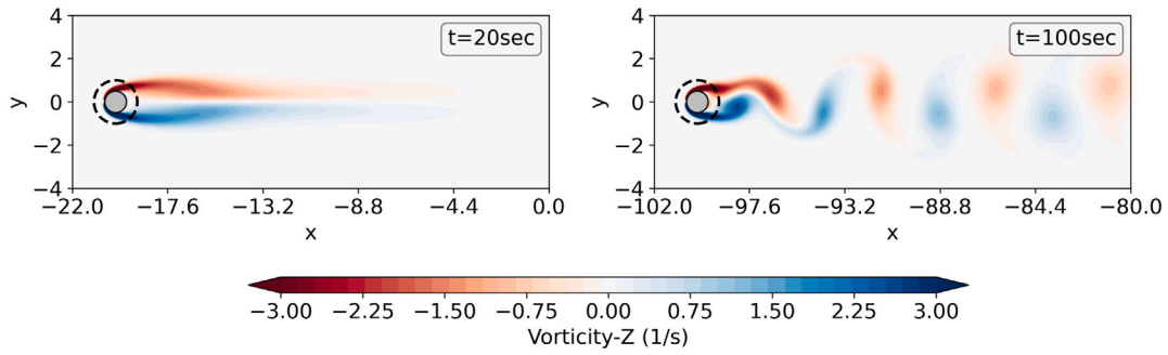
Fig. 11. Vorticity field for the case of the traveling cylinder at Re = 100 . The numerical boundary is represented with a black dashed circle line.
