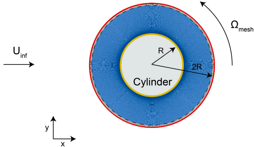
Fig. 12. The rotating cylinder case configuration. The cylinder rotates counterclockwise with a rotational speed \Omega_{mesh} , while a free-stream velocity U_{inf} acts in the +x direction.
