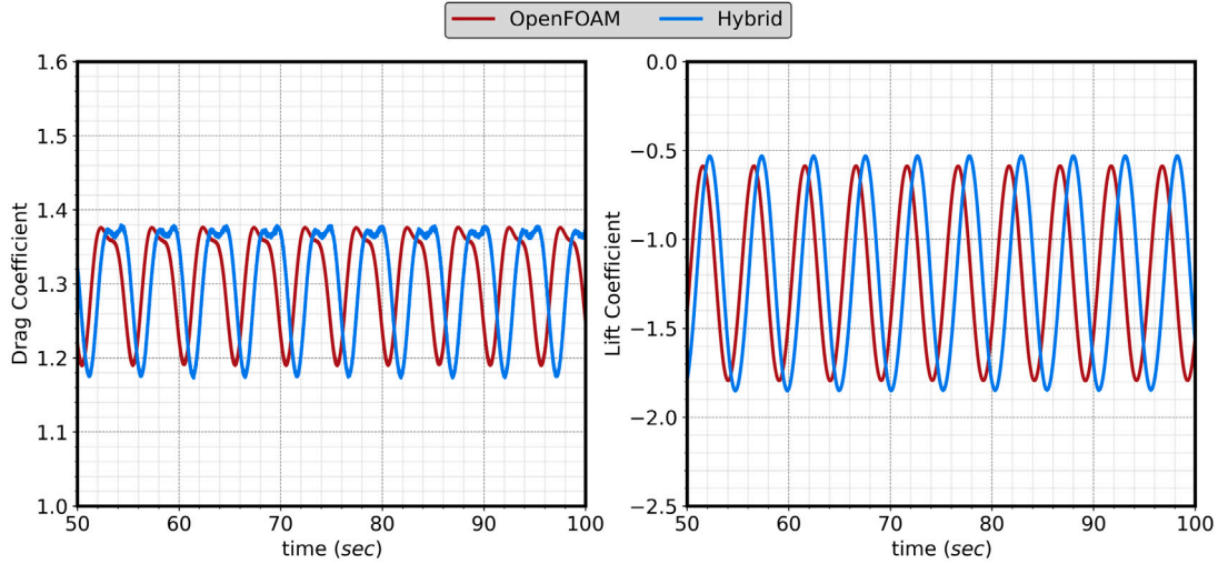
Fig. 13. Lift and drag coefficients over time for the case of the rotating cylinder at Re = 200 and \alpha = 0.5 .
