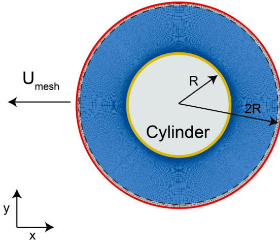
Fig. 5. The traveling cylinder case configuration. The cylinders moves in the -x direction with a constant velocity U_{mesh} .
