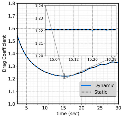
Fig. 9. Comparison of the drag coefficient between a static and a dynamic case where the mesh displacement is equal to the particles' spacing.
