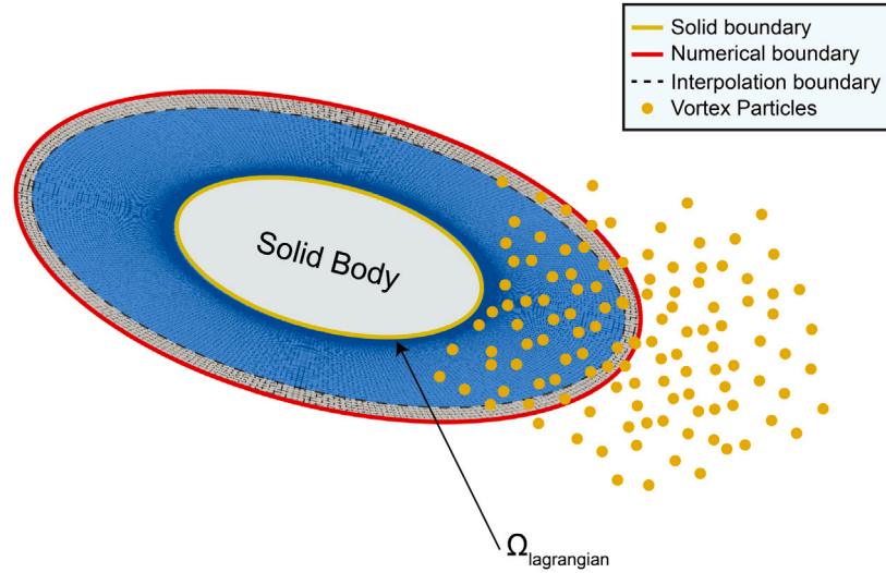
Fig. 1. Decomposition of the computational domain. The Lagrangian solver covers the entire computational domain (denoted as \Omega_{lagrangian} ), whereas the Eulerian mesh extends up to a short distance (numerical boundary) away from the solid boundary. The under-resolved solution of the Lagrangian is corrected using the Eulerian solution in a region bounded by the interpolation boundary.
