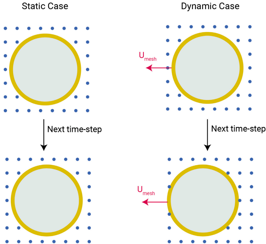
Fig. 7. Configuration of the Lagrangian particles close to the solid boundary over a time step. In the static case, the configuration remains the same; for the dynamic case, the distribution of the particles around the solid boundary changes, leading to high-frequency oscillations in the calculation of the Eulerian boundary conditions and, subsequently, on the body forces.
