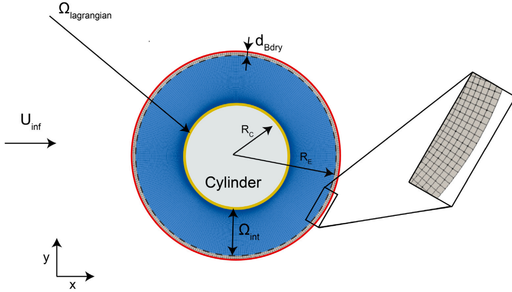
Fig. 4. The cylinder configuration used for the validation cases, with a snippet depicting the cells close to the numerical boundary.
