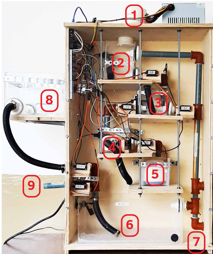
FIG. 5.55 System layers, photograph of one of two implemented prototypes.
