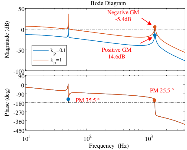
Fig. 4. Control loop without active damping (a) Poles-zeros map (b) Bode Plot.
