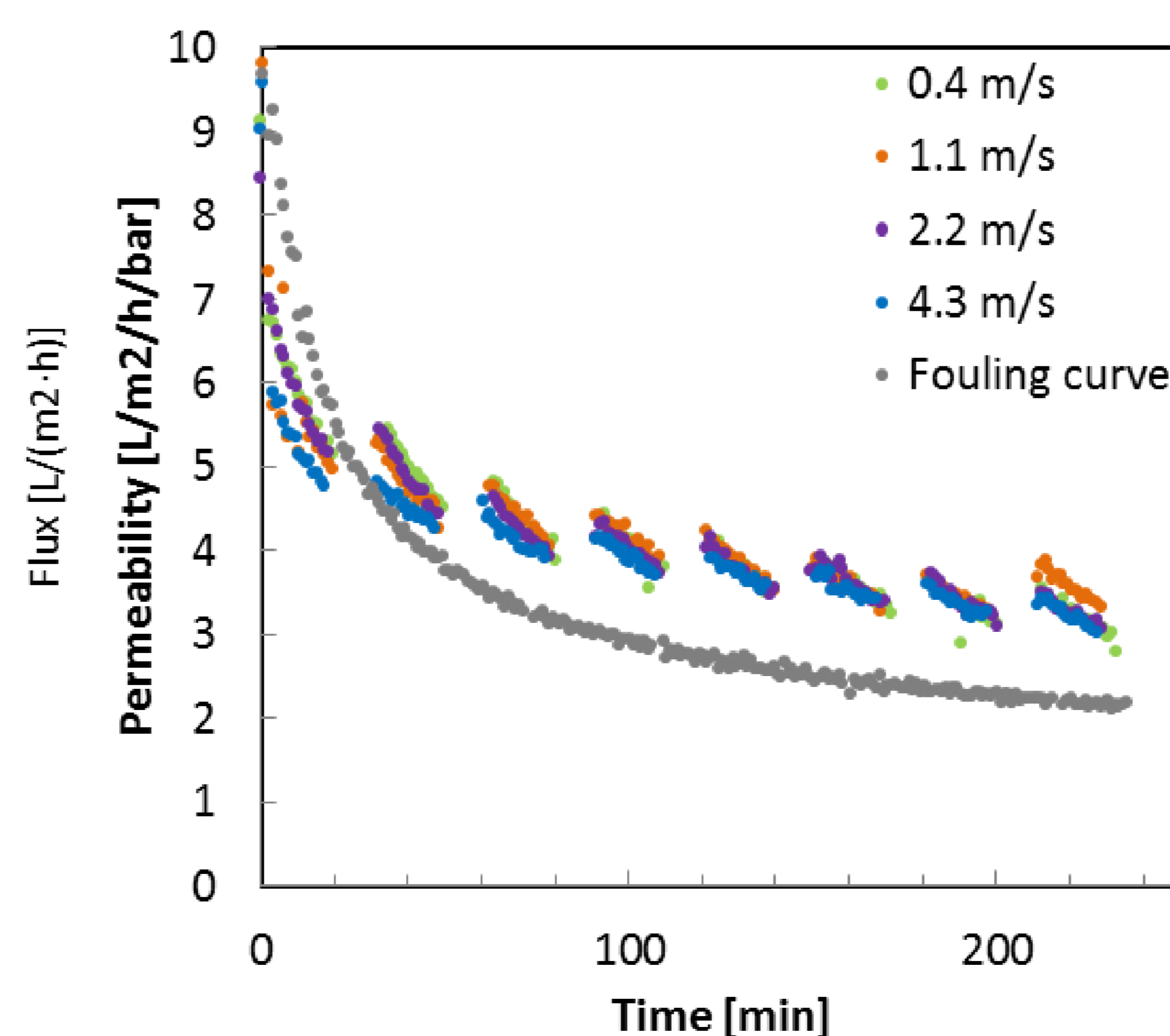
Figure 3: Permeability in time of ceramic NF with and without interval forward flush (20 min). Different crossflow velocities for forward flush are shown.
