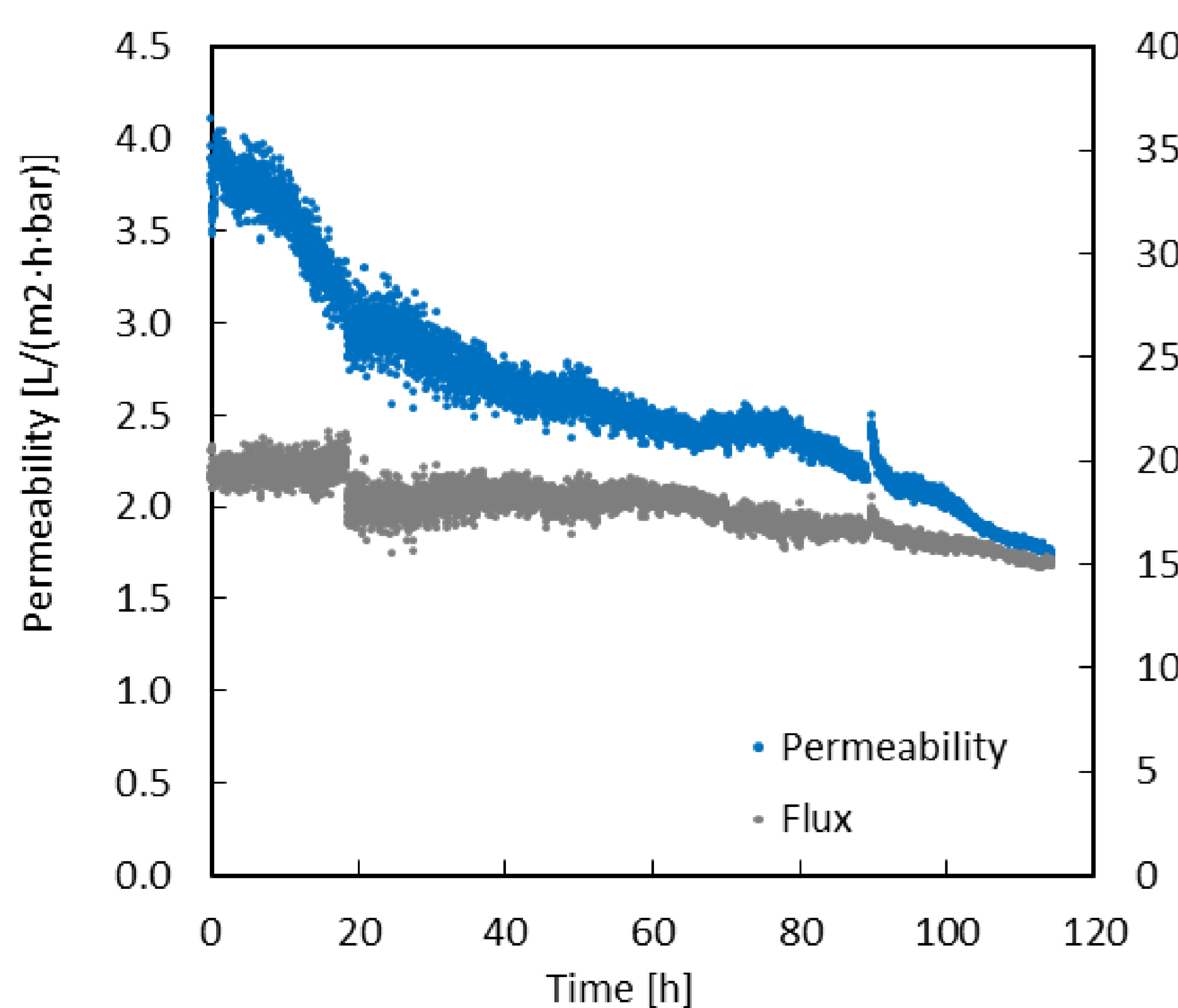
Figure 2: Permeability and flux in time of ceramic NF using pre-sieved domestic wastewater. Duration of 5 days without cleaning the membranes*.
