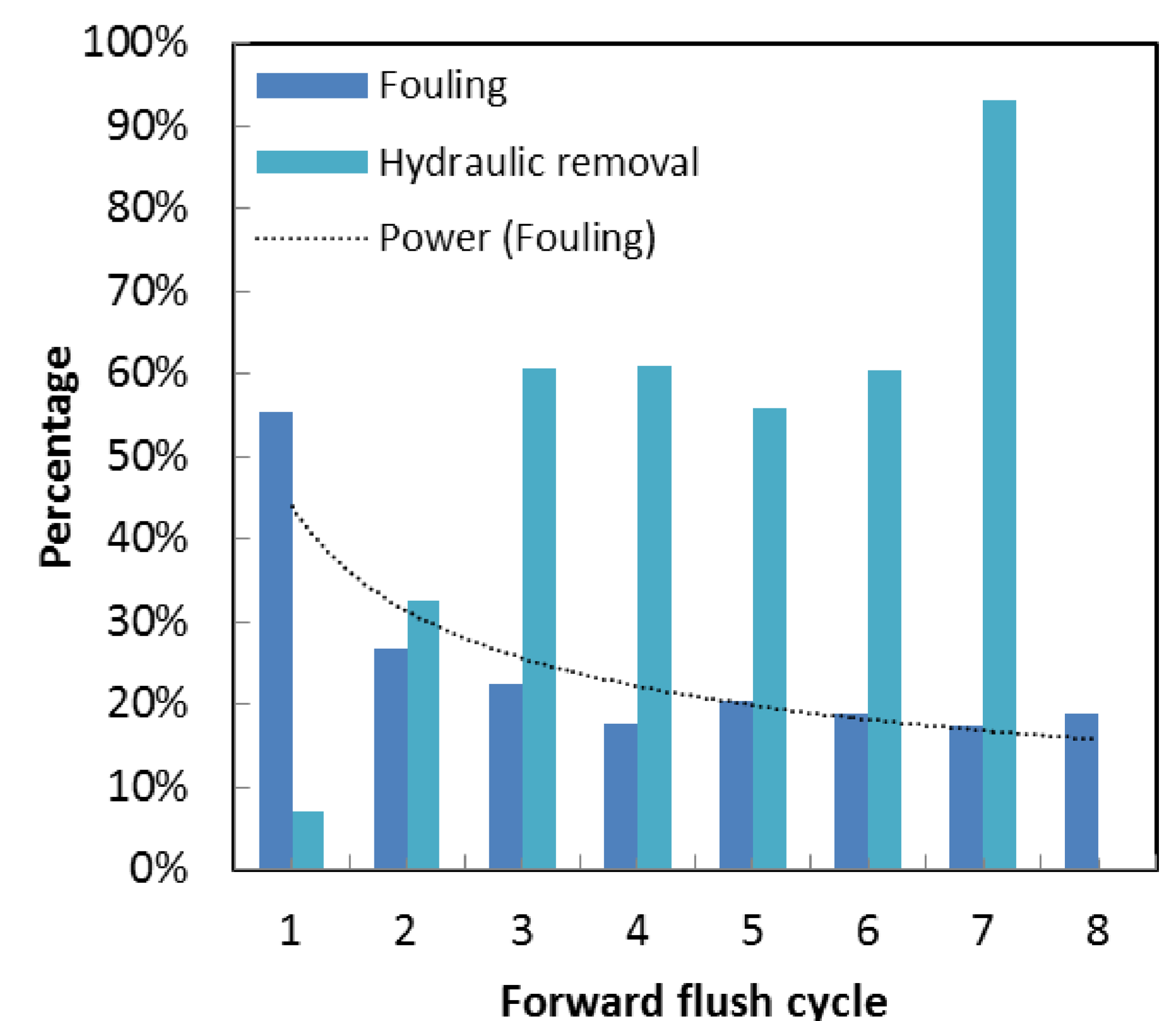
Figure 4: Fouling and hydraulic removal per forward flush cycle. Forward flush cycles of 20 minutes were executed.
