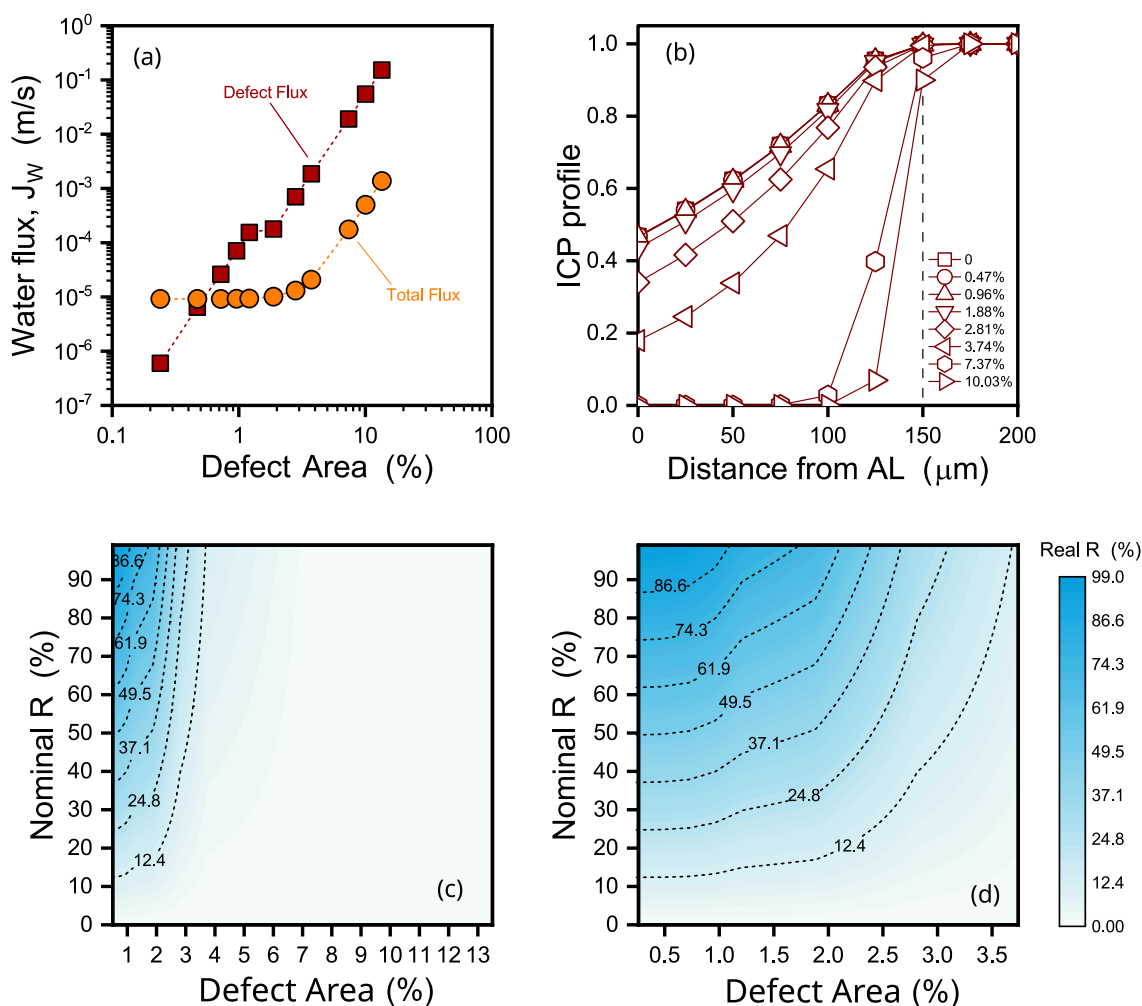
Fig. 6. Influence of the presence of defects on the AL on membrane performances. Results present a) the water flux through the membrane as function of the increase of the defected area in AL. Water flux is distinguished between defected and total flux, thus incorporating both the convective flux through the defected area and the water passage through the AL, via solution–diffusion. The related ICP profile is reported in b), as function of the distance from the active layer. The contour-plot c) shows the real rejection of a TFC-FO membrane while varying its nominal selectivity (e.g., declared by the membrane manufacturer) as function of the possible presents of defects on the AL. A zoom into the most relevant area is shown in d).
