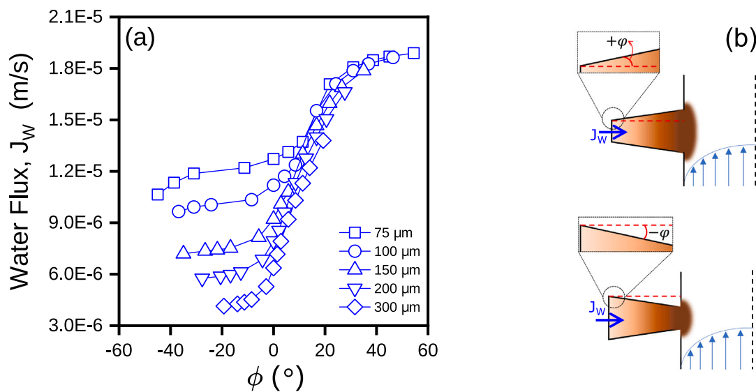
Fig. 4. Influence of porous support (i) geometry and (ii) thickness on water flux through the membrane. Results of the CFD simulations are reported in a) showing the water flux J_w as function of a sensitivity analysis performed to investigate b) widening/narrowing conical pore geometries while varying the thickness of the porous support. \square , \circ , \Delta , \nabla and, \diamond refer to different porous support thicknesses and not to the pore shape as reported in previous figures. Orange and blue bars reported in d) are representative of the water flux modelled by considering (orange) or not (blue) the reverse salt flux in the CFD simulations.
