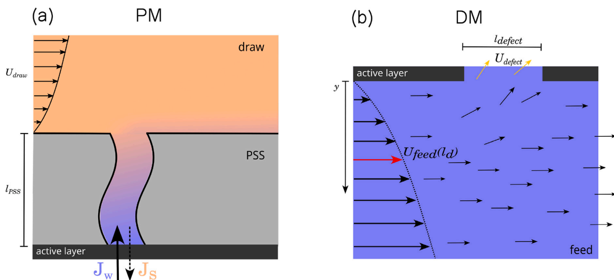
Fig. 2. (a) Porous Model represented by a single pore geometry. Blue and orange arrows represent the water and the reverse salt fluxes through the AL, respectively. The figure is reporting the curved shape, indicated with \nabla within the text. Alternative shapes were investigated and indicated as follows: straight \square , narrowing cone \Delta , widening cone \diamond , concave cone \circ and convex cone \ominus . (b) Resolution of the Defect Model in the vicinity of the defect in the AL. The arrows indicate the local cross flow of water within the feed channel and the convective flow through the defect.
