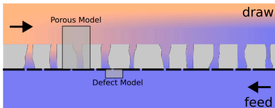
Fig. 1. Schematic representation of the draw and feed channel with a porous support (grey) and an active layer (black) in a counter cross-flow setup. The draw solute gets diluted along the draw channel and inside the support pores (ICP). The two rectangles indicate the two models of this study: The Porous Model is used to investigate the influence of the porous support geometry, as well as the effect of (i) the reverse salt flux and (ii) the draw cross flow velocity on the ICP and the relative water flux through the AL. The Defect Model quantifies the potential contamination of the draw side ascribed to the convective passage of flow from the feed to the draw channel due to the presence of a defected Active Layer.
