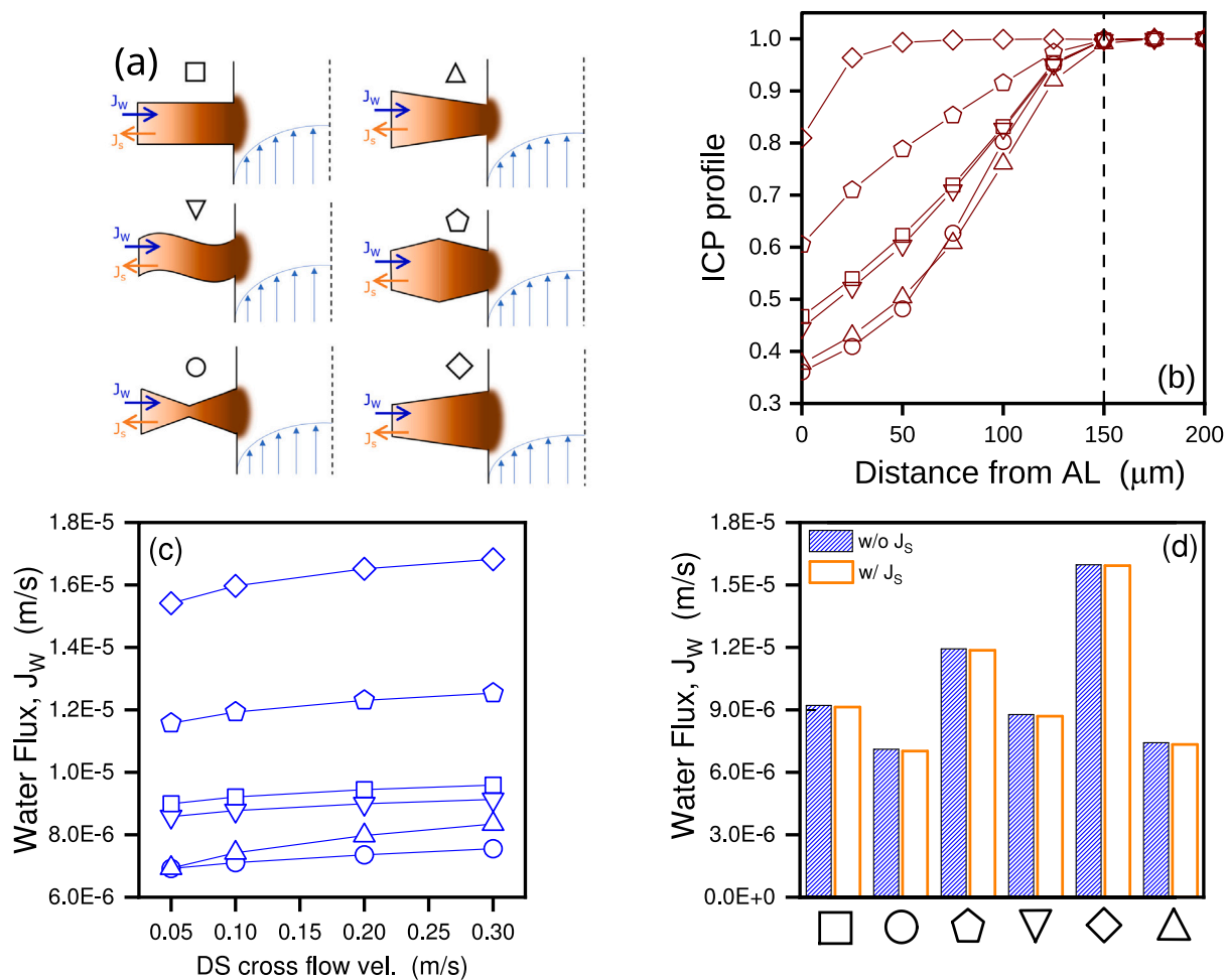
Fig. 3. Influence of porous support structure and DS operating parameter on ICP and water flux in FO membrane. (a) Sketch of different support geometries, indicating solute dilution towards draw channel, (b) resulting ICP profile along support towards draw channel, (c) water flux in dependence of the cross flow velocity, (d) influence of the reverse salt flux on the water flux is presented in as function of the different porous support geometries.
