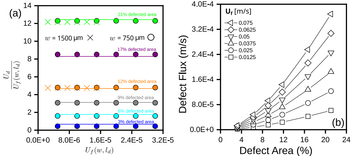
Fig. 5. (a) Relation of relative defect flow U_d/U_f and near-wall cross flow U_f and its dependence on the defect area and feed channel width. The circles and crosses refer to the feed channel width w , while the different colours indicate different values of the defect length l_d (and hence the defect area). The solid lines follow the scaling law (2). b) Effect of cross flow velocity and defect area on defect flux, according to Eq. (3). The defect flow is proportional to the bulk cross flow velocity, while it scales with the 1 + \sqrt{2} power of the defect length l_d . It is seen that the defect flux may assume a one order of magnitude greater flux than osmotic flux, for reasonably small defect areas.
