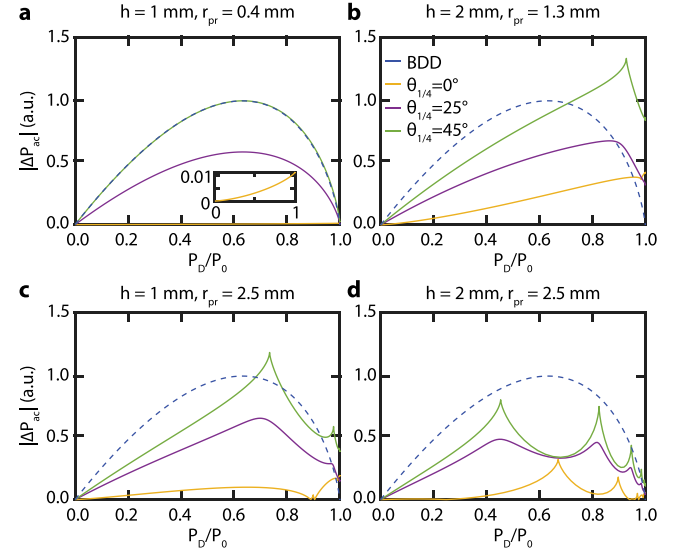
Fig. 8. Calculated absolute CI sensitivity |\Delta P_{ac}| for \theta_{1/4} = 0^\circ (yellow), 25^\circ (purple), 45^\circ (green) and for different values of r_{pr} and h : a h = 1 mm and r_{pr} = 0.4 mm, b h = 2 mm and r_{pr} = 1.3 mm, c h = 1 mm and r_{pr} = 2.5 mm, and d h = 2 mm and r_{pr} = 2.5 mm. The intensities are normalized w.r.t. the maximum of the BDD sensitivity shown by dashed blue line. The inset in panel a shows a zoom of the \theta_{1/4} = 0^\circ case. (For interpretation of the references to color in this figure legend, the reader is referred to the web version of this article.)
