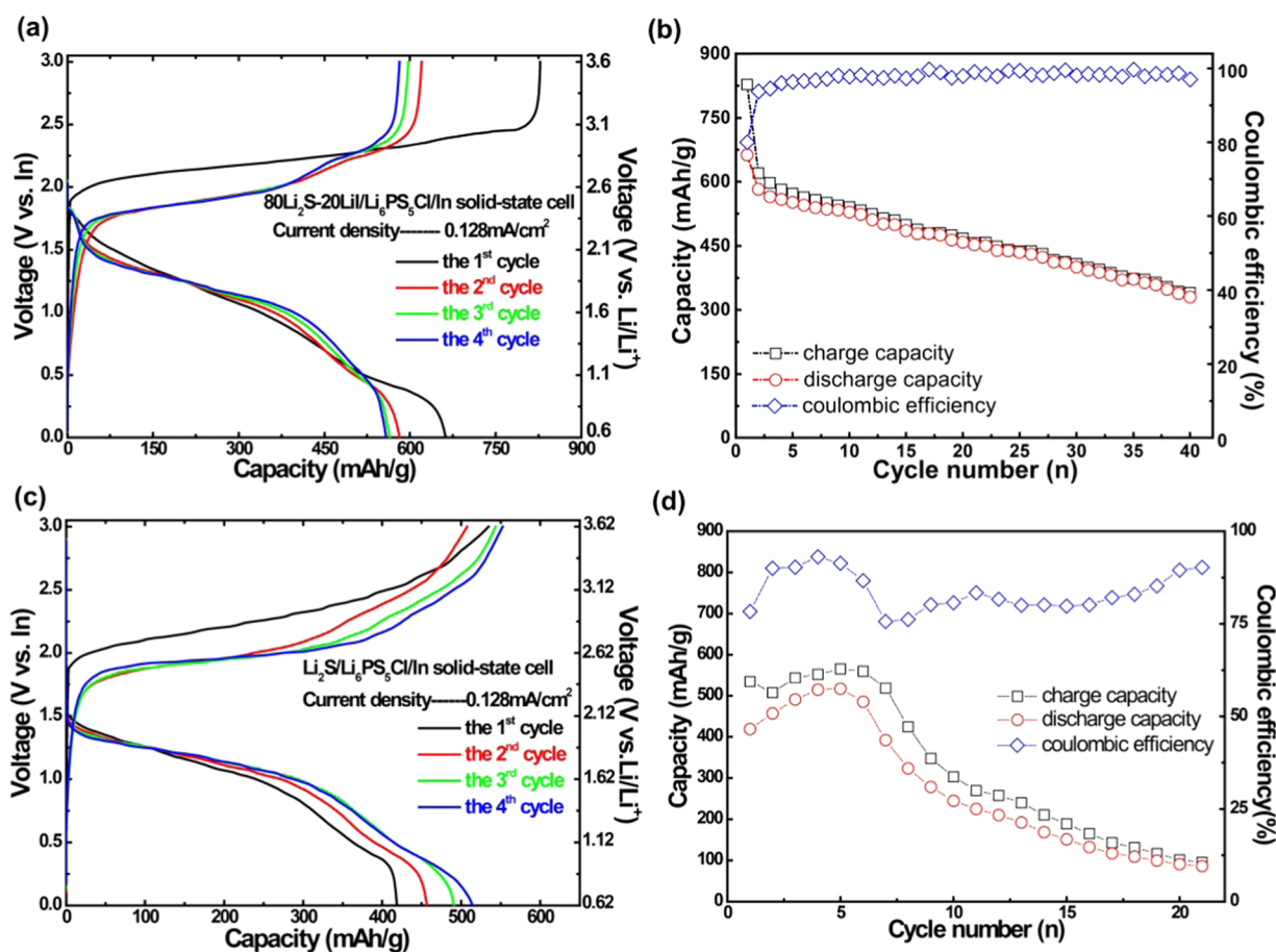
Figure 6. First four (dis)charge curves and the cycling performances of all-solid-state batteries 80\text{Li}_2\text{S}-20\text{Li}/\text{Li}_6\text{PS}_5\text{Cl}/\text{In} (a, b) and \text{Li}_2\text{S}/\text{Li}_6\text{PS}_5\text{Cl}/\text{In} , based on the SSM- \text{Li}_6\text{PS}_5\text{Cl} material annealed at 550\text{ }^\circ\text{C} , (c, d) measured at a current density of 0.128\text{ mA cm}^{-2} applied between 0 and 3.0 V vs In ( 0.62\text{--}3.62\text{ V vs Li}^+/\text{Li} ).
