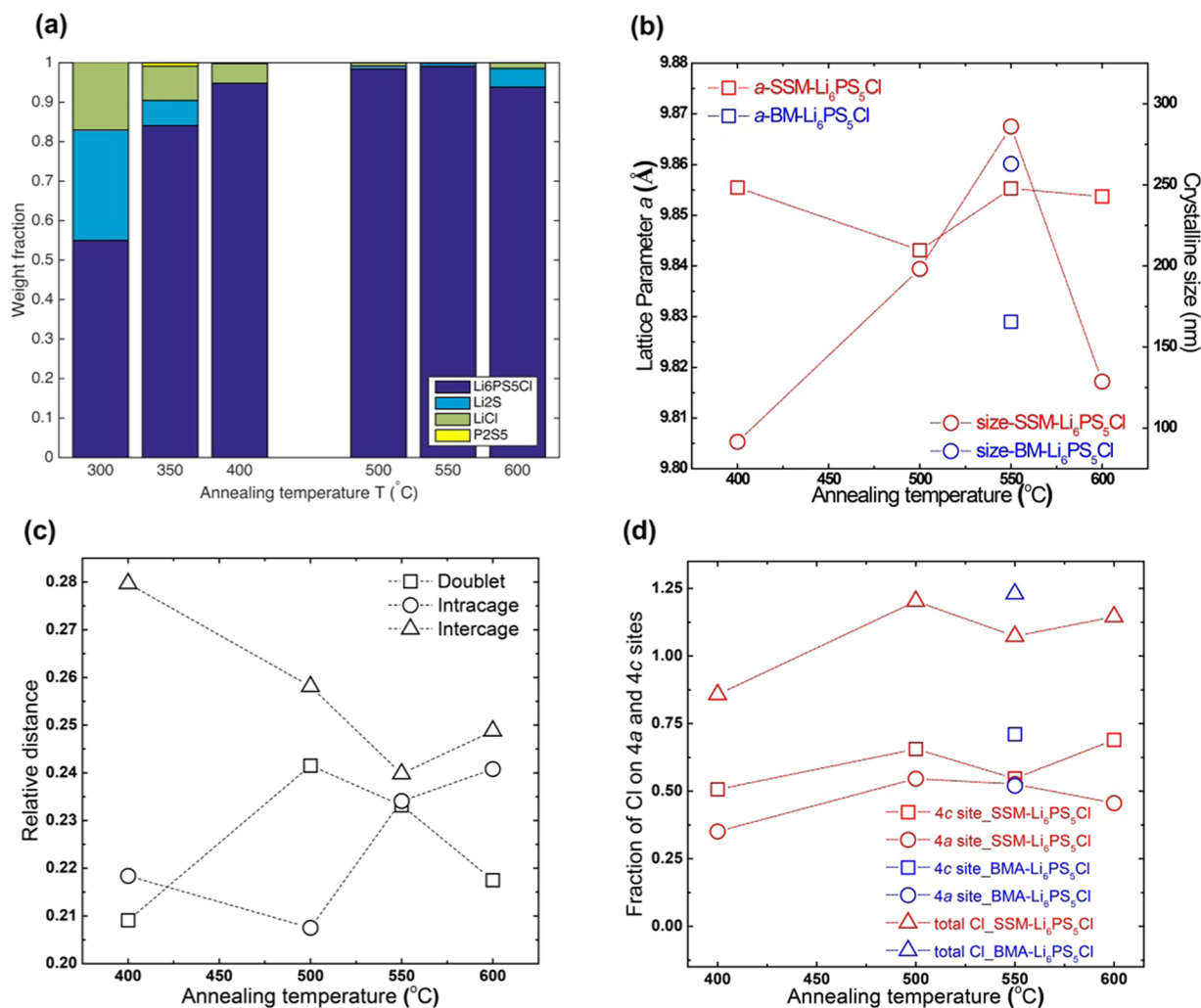
Figure 3. (a) Phase fractions from XRD refinement of SSM- \text{Li}_6\text{PS}_5\text{Cl} annealed at various temperatures (300, 350, 400, 500, 550, and 600 °C). (b) The crystallite size and lattice parameters, all resulting from simultaneous refinement of the XRD and ND patterns of SSM- \text{Li}_6\text{PS}_5\text{Cl} obtained after various annealing temperatures and of the conventionally prepared BMA- \text{Li}_6\text{PS}_5\text{Cl} material (by mechanical milling followed by annealing). (c) Inter-cage, intra-cage, and doublet relative jump distance of Li-ions of SSM- \text{Li}_6\text{PS}_5\text{Cl} annealed at various temperatures. (d) the distribution of Cl on the 4c and 4a sites and the total Cl composition.
