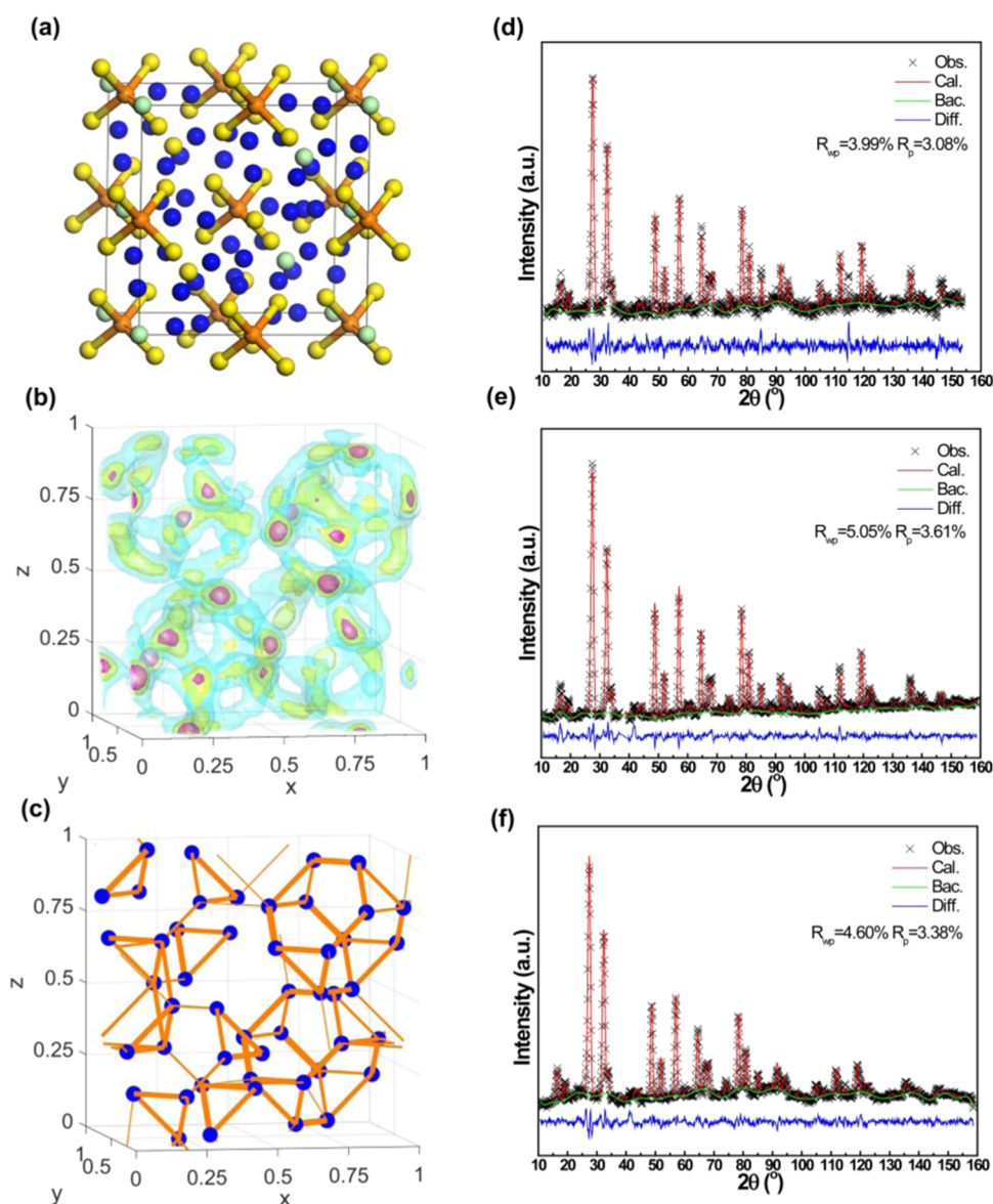
Figure 2. (a) Unit cell of argyrodite \text{Li}_6\text{PS}_5\text{Cl} in the \overline{F}43m space group. Blue spheres represent Li atoms, orange represents phosphorous, yellow represents sulfur, and green represents chloride atoms. (b) Li-ion density of \text{Li}_6\text{PS}_5\text{Cl} at 500 K during a DFT-based MD simulation demonstrates the diffusion pathway. The red surfaces correspond to higher Li-ion densities and blue surfaces to lower densities. The x , y , and z coordinates are given in fractional coordinates. (c) The jump statistic plot between different Li sites resulting from the DFT-based MD simulation shown in (b). The blue spheres indicate the 48h Li sites in the \overline{F}43m group. The orange lines indicate jumps between the lattice sites. Thicker lines indicate higher jump rates. Neutron diffraction patterns including their Rietveld refinement for the pristine SSM- \text{Li}_6\text{PS}_5\text{Cl} material prepared by annealing at various synthesis temperatures: (d) 500 °C, (e) 550 °C, and (f) 600 °C.
