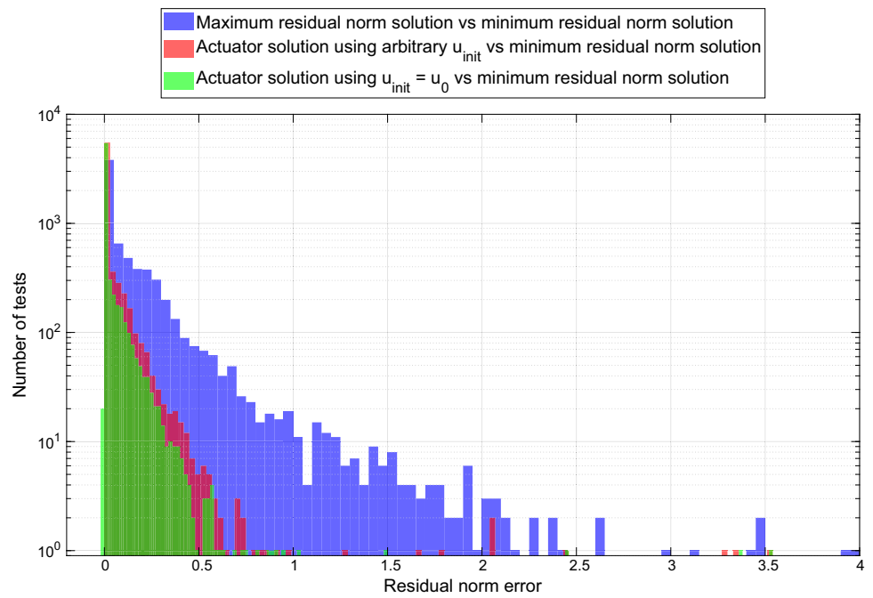
Fig. 15 Residual norm error between the minimum residual norm solution and the solution computed using different u_{init} conditions. Notice that the y-axis is logarithmic and some points are not fully represented. One point of the red histogram and four points of the blue histogram are above the residual norm error of 4. These points are mentioned in the Statistical analysis results Section
