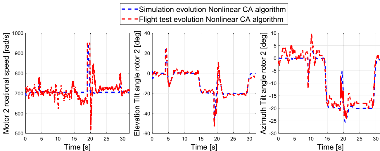
Fig. 11 Tilting angles and motor rotational speed evolution of rotor number 2 computed by the Nonlinear CA algorithm. The dashed blue curve is the simulated actuator evolution while the dashed red curve is the actuator evolution experienced during the flight test
