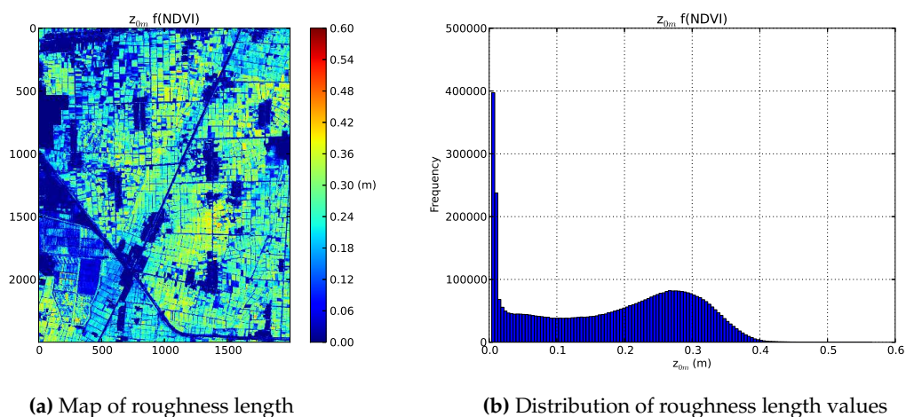
Figure 3. (a) Map and (b) frequency distribution of roughness length for momentum transfer values over the Yingke oasis station following Moran's formulation.
