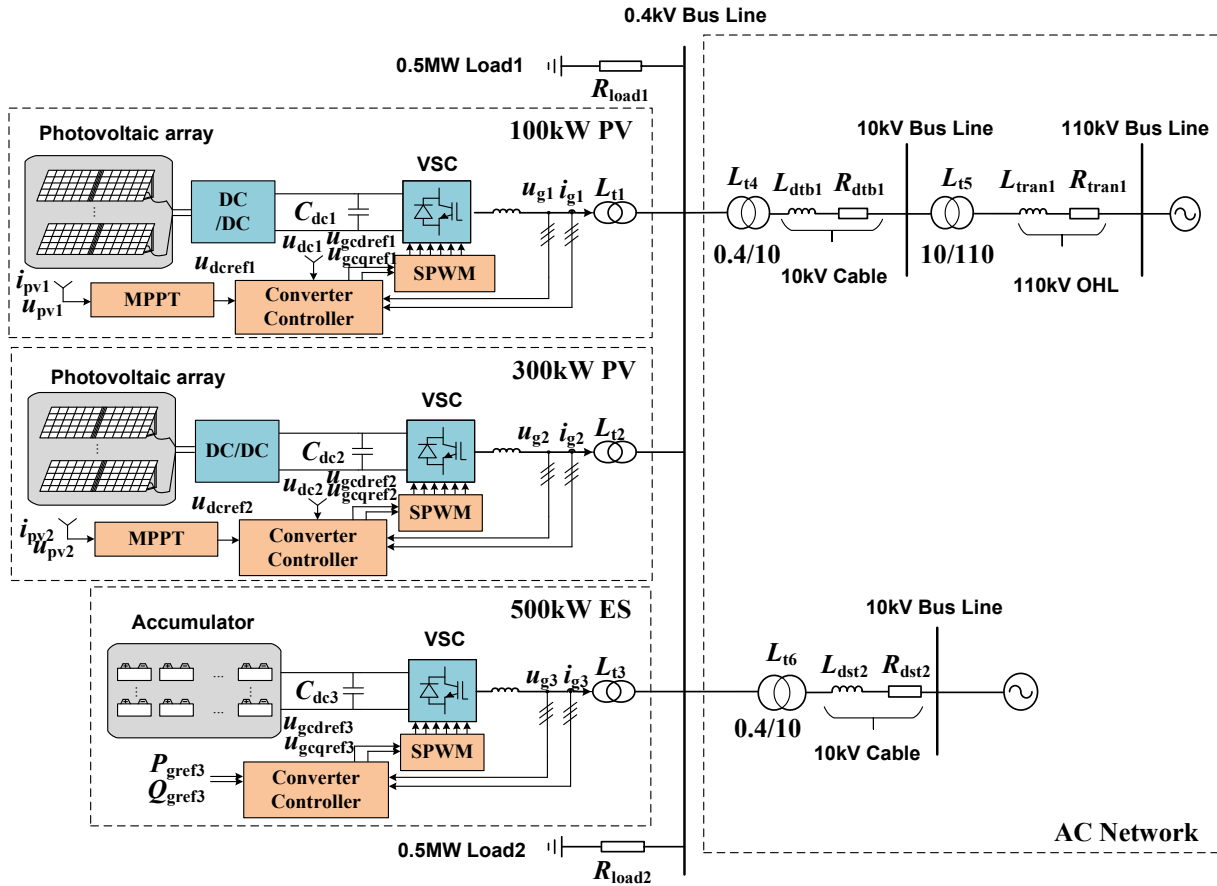
Fig. 11. Connection structure diagram of the ADN with PVs and ES.
