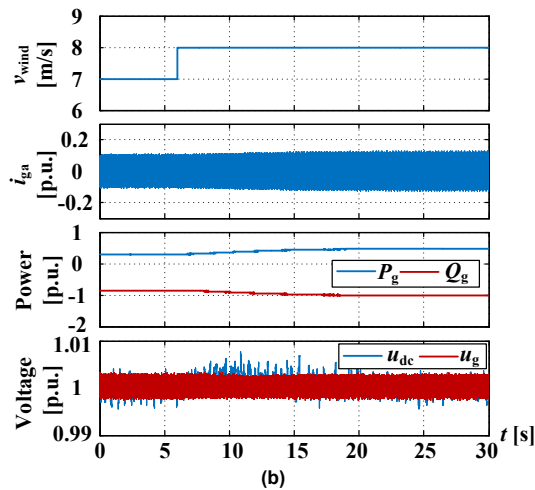
Fig. 16. Generation process of supplementary current signals in CSI-ECSC.
