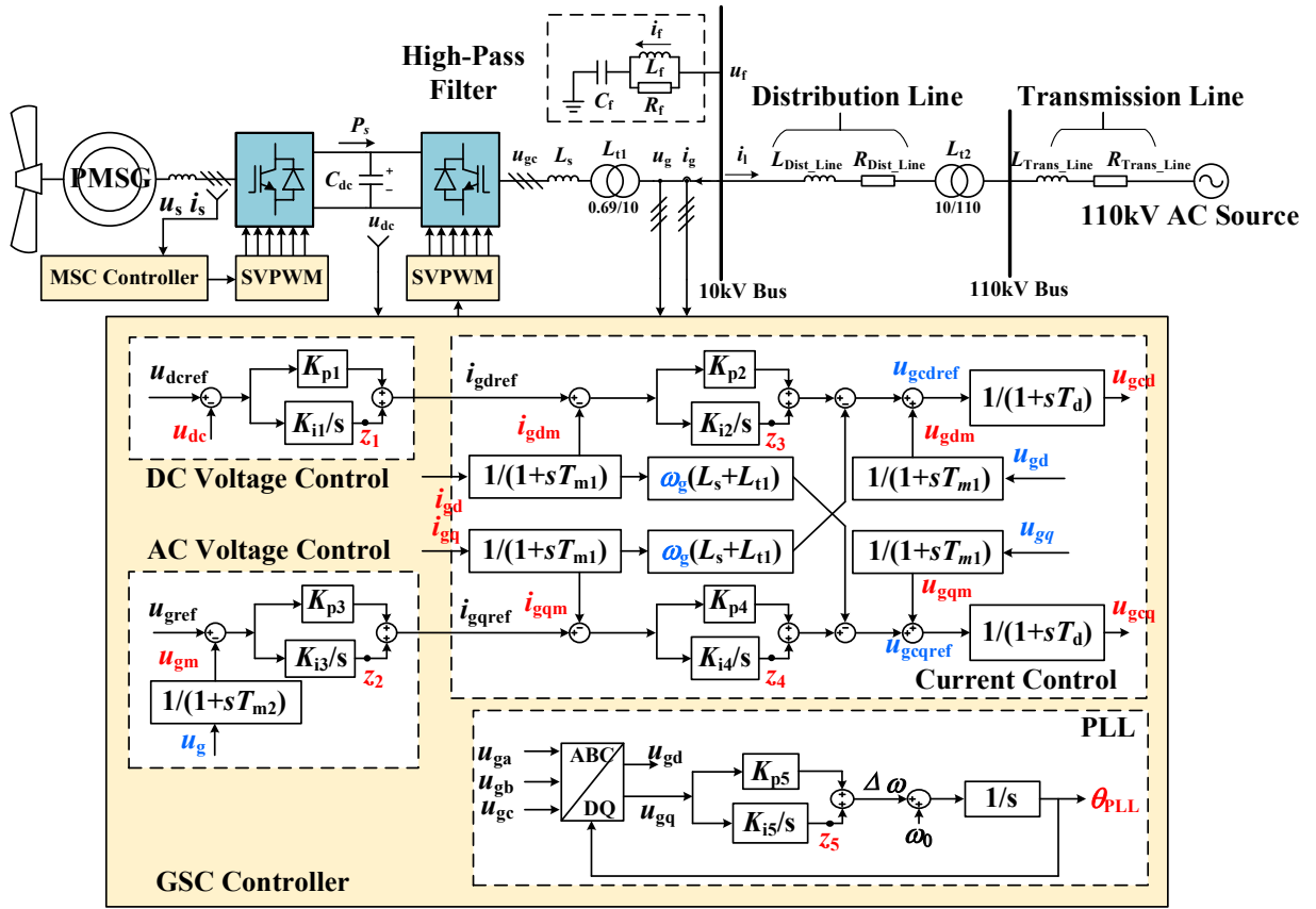
Fig. 1. Connection structure diagram and control system of the target system.
