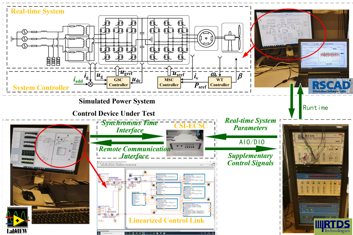
Fig. 14. The general structure of HIL testing on developed CSI-ECSC and physical picture of the HIP testing platform.
