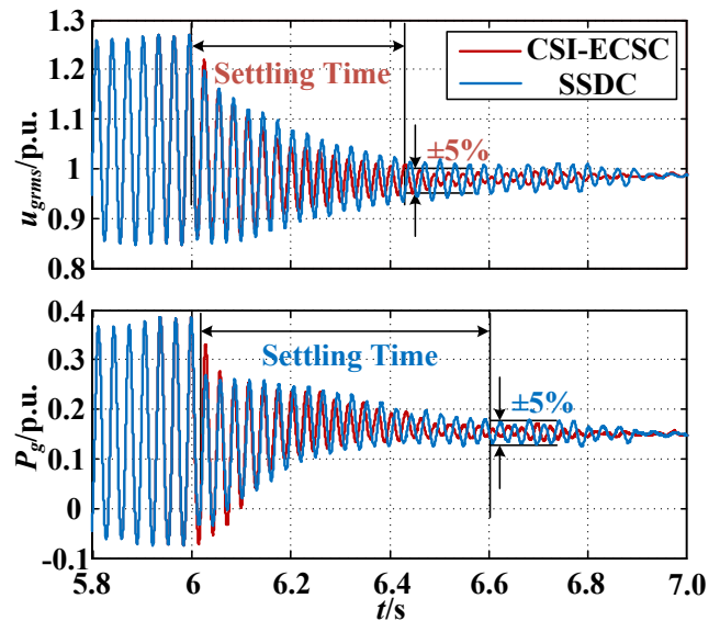
Fig. 10. Waveforms of u_{grms} and P_g at PCC of the system comparison between CSI-ECSC and SSDC.
