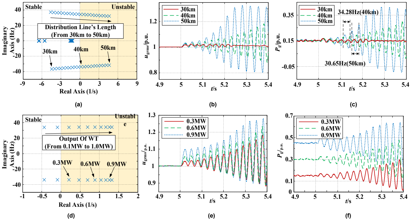
Fig. 3. Root loci in theory and waveforms in simulation (a) Root loci as length of distribution line changes, (b) Waveforms of effective value of AC voltage u_{grms} at PCC as length of distribution line changes, (c) Waveforms of effective value of active power P_g at PCC as length of distribution line changes, (d) Root loci as output power of WT changes, (e) Waveforms of effective value of AC voltage u_{grms} at PCC as output power of WT changes, (f) Waveforms of effective value of active power P_g at PCC as output power of WT changes.
