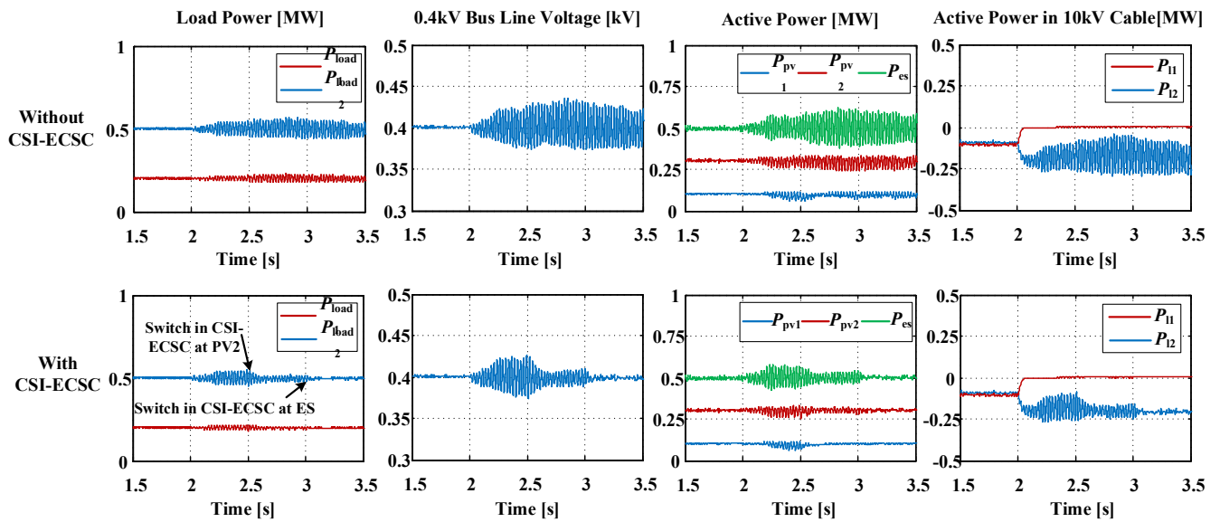
Fig. 13. Waveforms of load power, 0.4 kV bus line voltage, active power of each units, and active power in 10 kV cable are drawn with and without CSI-ECSC in simulation.
