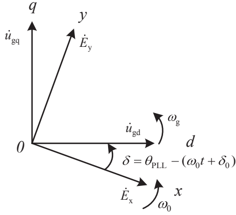
Fig. 2. Vector graph of coordinate transformation between the synchronous rotating coordinate system of GSC and that of infinite system.
