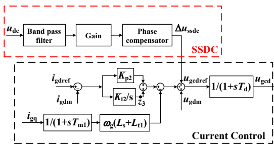
Fig. 9. SSDC scheme in the GSC controller.
