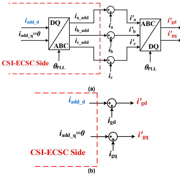
Fig. 6. Equivalent process of supplementary current signal coupling, (a) Actual block diagram of supplementary current signal coupling, (b) Equivalent block diagram of supplementary current signal coupling.
