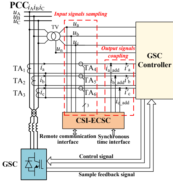
Fig. 5. Hardware interface circuit of CSI-ECSC.
