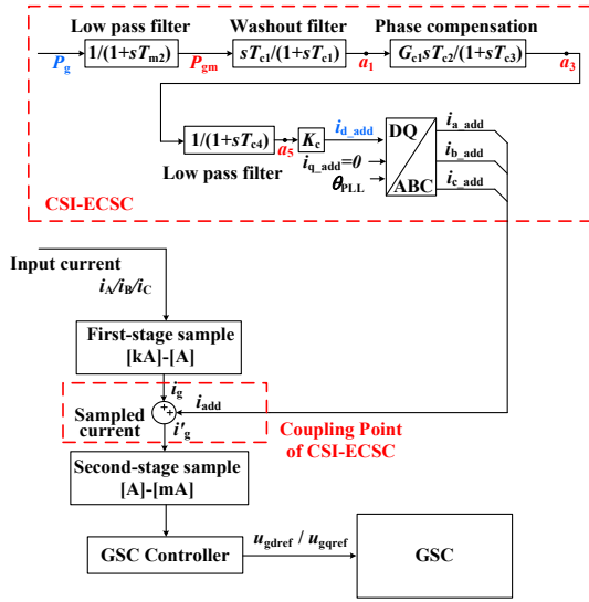
Fig. 4. CSI-ECSC scheme outside the GSC controller.
