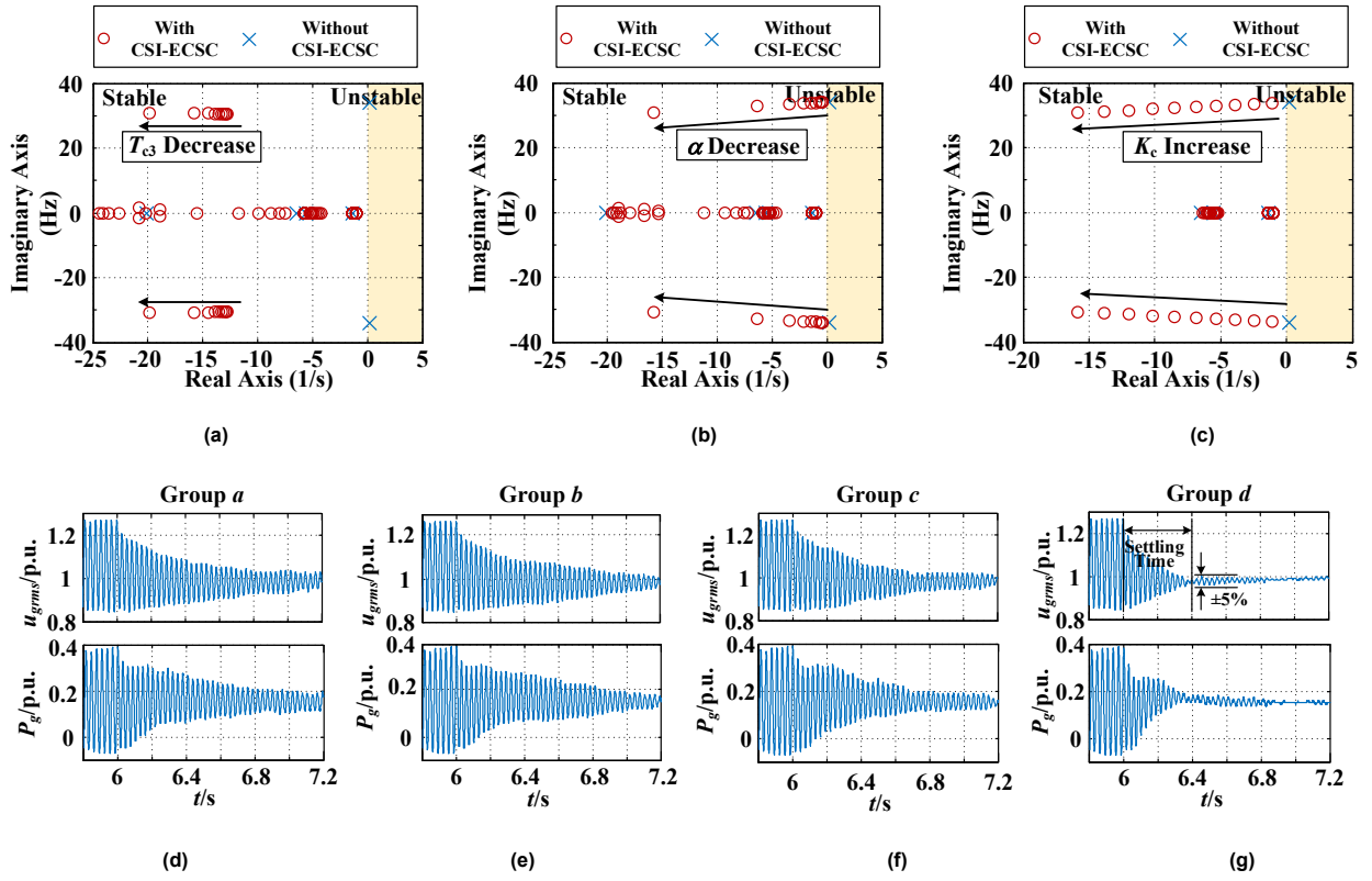
Fig. 8. Root loci and waveforms of u_{grms} and P_g at PCC of the system with CSI-ECSC under variation of key parameters, (a) Root loci under T_{c3} changes, (b) Root loci under \alpha changes, (c) Root loci under K_c changes, (d) Waveforms of u_{grms} and P_g at PCC under variation of key parameters.
