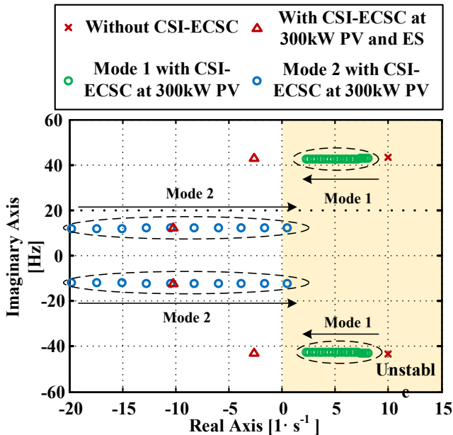
Fig. 12. Leading root loci of the ADN with PVs and ES.
