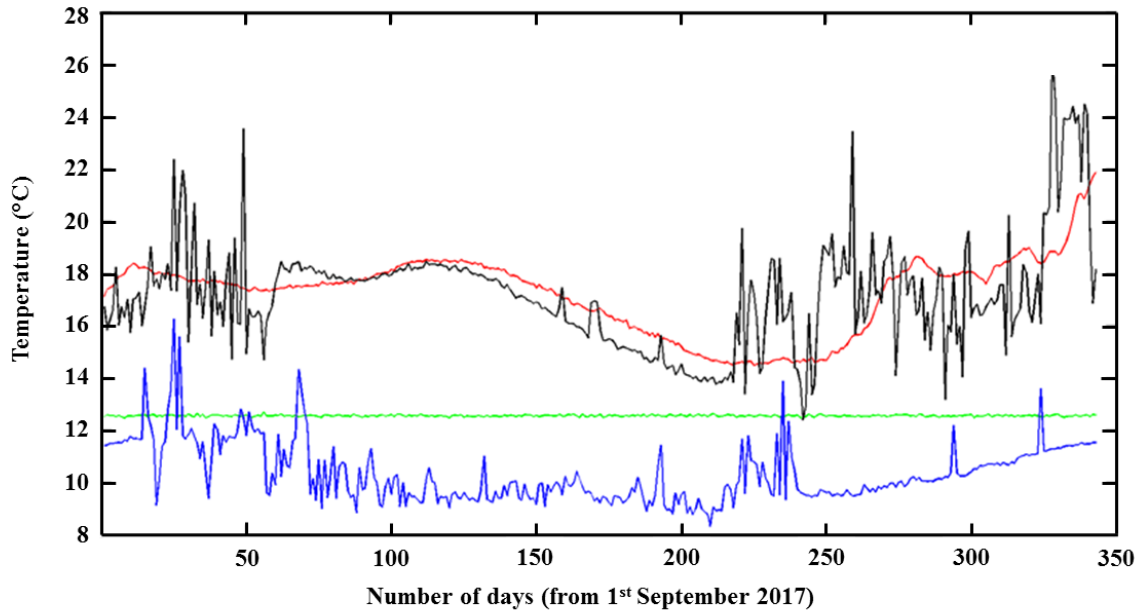
348 Figure 7. Temperature evolution in days after 1 September 2017 (day zero) at 80m depth for the 4 different wells in Ham. Monitoring 349 well 1 is situated at 10 m downstream from the hot well (production well 1). Monitoring well 2 is situated further downstream between 350 the hot and the cold well.
