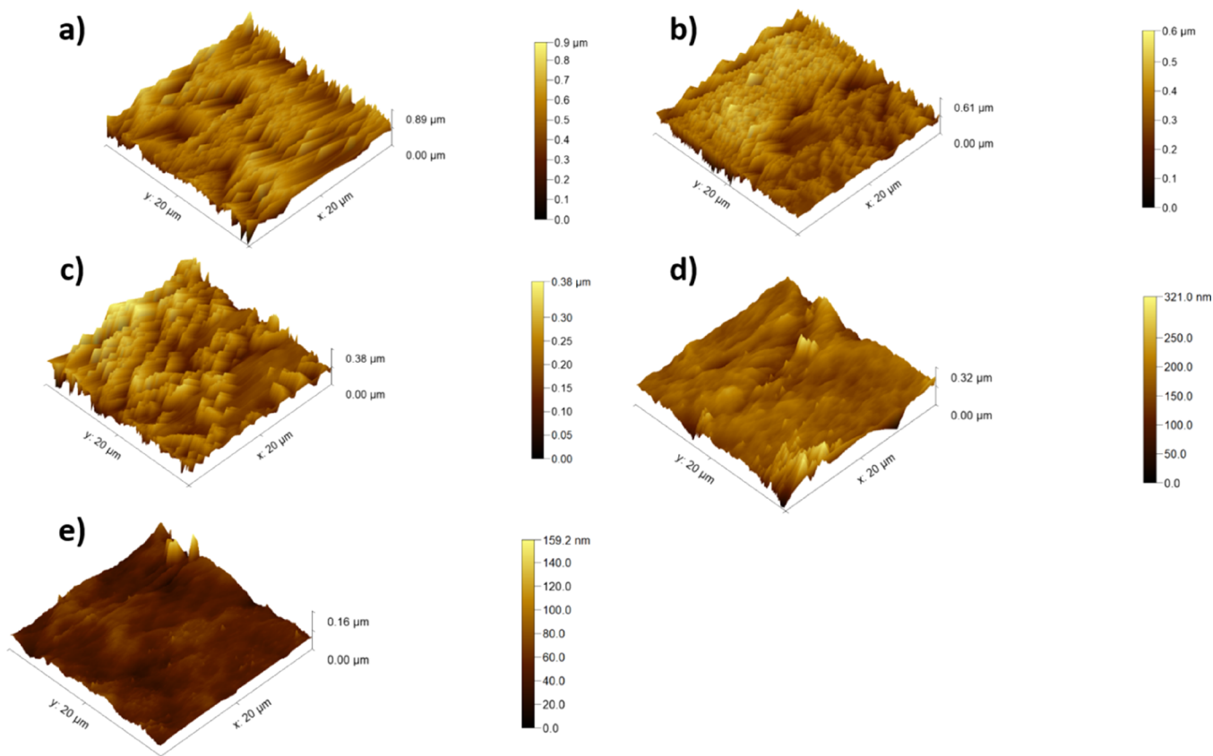
Figure 3. 3D AFM images of PVDF (a) and composites with 2 wt % of nanofillers NDM (b), NDO (c), NDA (d), and NDH (e).
