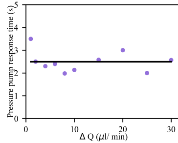
(b) Pump response time for different flow rate variations, \Delta Q
