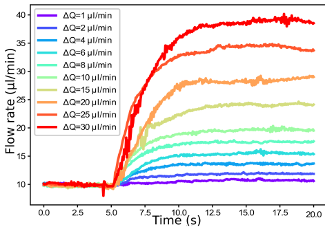
(a) Flow rate variations as a function of time where the flow rate is kept constant 10 \mu\text{l}/\text{min} from 0 to 5 secs for all the test cases. At t = 5 secs, a new input value is transmitted to the pump. The experiment is repeated for multiple flow rate variations.
