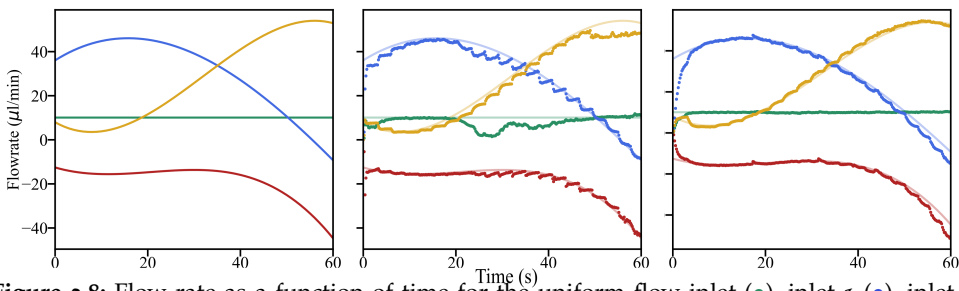
Figure 3.8: Flow rate as a function of time for the uniform flow inlet ( \bullet ), inlet 1 ( \bullet ), inlet 2 ( \bullet ) and inlet 3 ( \bullet ). (A) pre-defined output (B) pre-defined output (solid lines); experimentally measured flow rates from the pump without modeling the pump response time to the input flow rate (dotted lines). (C) pre-defined output (solid lines); experimentally measured flow rates from the pump for the modified input where the input is modeled with the pump response time (dotted lines).
